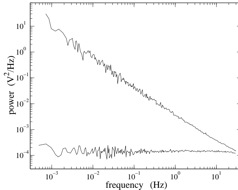
Figure 3.3. Noise in a 50\ \Omega resistor with and without a current
