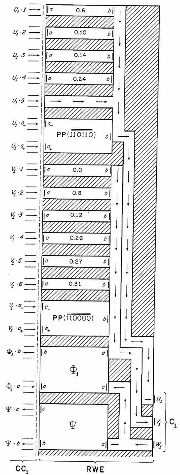
Fig. 39. Read-write-erase unit RWE. (a) Upper part of RWE
