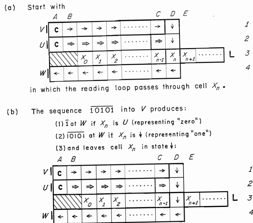
Fig. 51. New method of operating the linear array L
