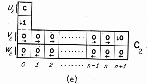
Fig. 32. Lengthening the timing loop C_2
