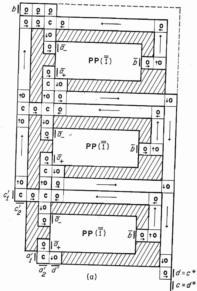
Fig. 24. Design of triple-return counter \Phi
