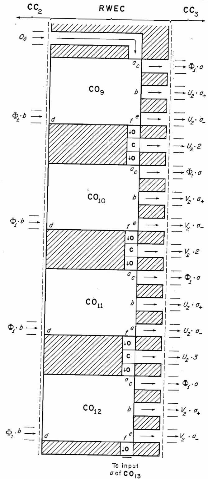
Fig. 41. Read-write-erase control RWEC. (d) Control organs for shortening C_2 . (This figure is continued from p. 360.)
