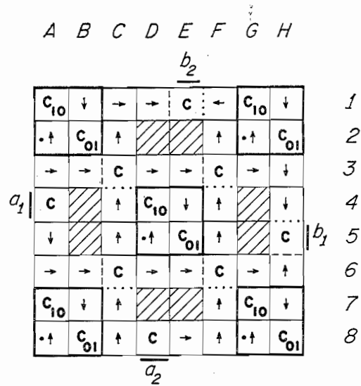
(a) Crossing organ
