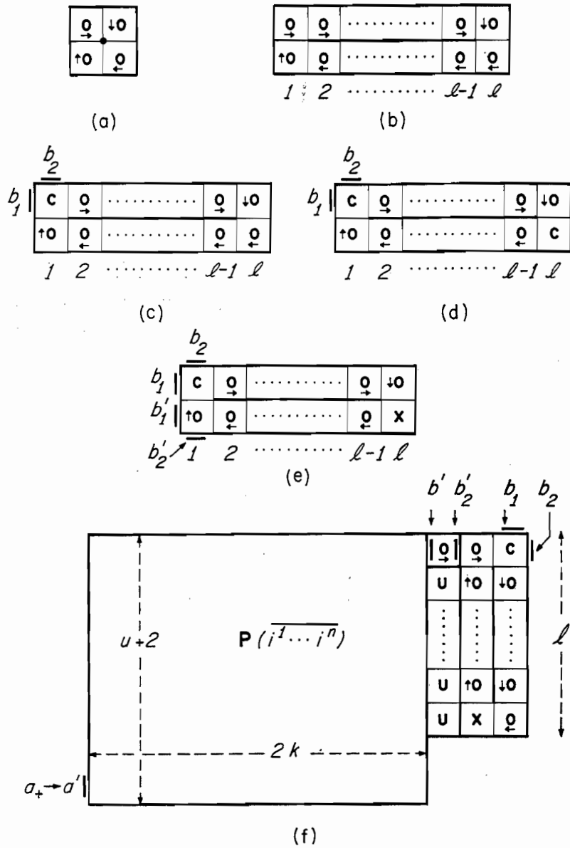
Fig. 18. Design of a periodic pulser: initial construction
