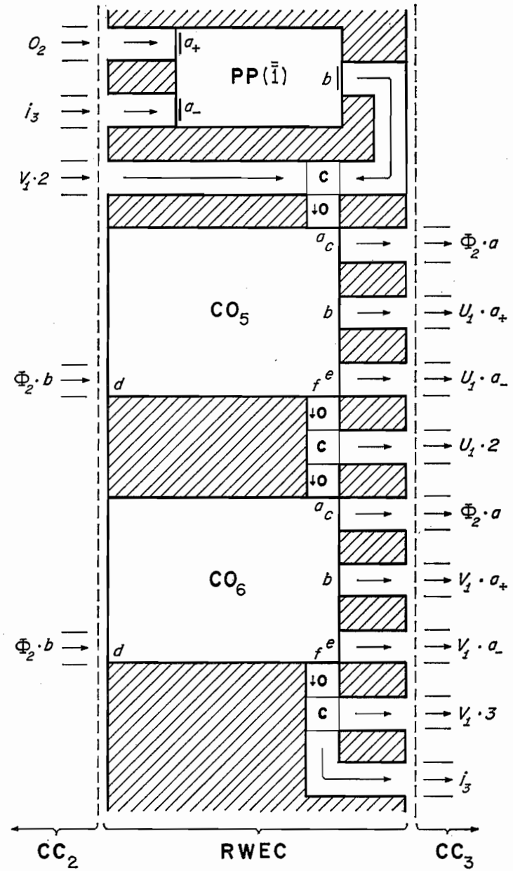
Fig. 41. Read-write-erase control RWEC. (b) PP(\bar{1}) to store the fact that a "zero" is to be written in x_n , and control organs for writing a zero and lengthening the upper part of C_1 . (This figure is continued from p. 358.)
