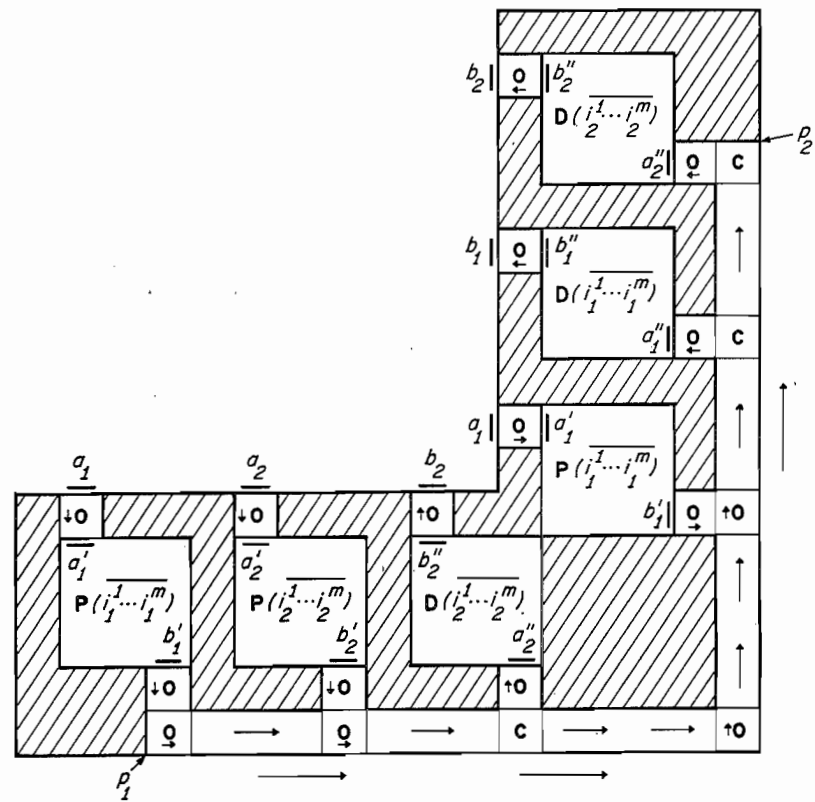
Fig. 29. Pulsers and decoders of a coded channel
