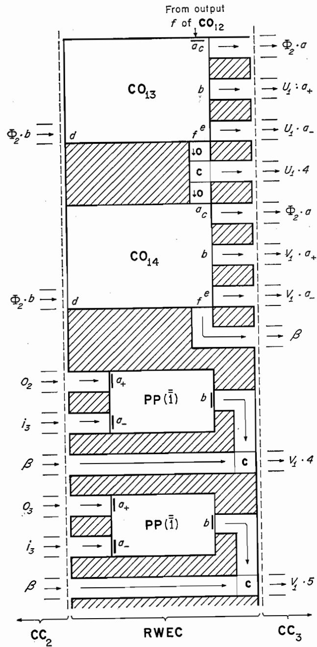
Fig. 41. Read-write-erase control RWEC . (e) Control organs and PP(\bar{i}) for shortening the lower part of C_1 and writing in cell x_n . (This figure is continued from p. 361.)
