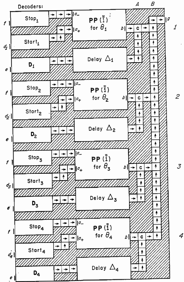
Fig. 53. Static-dynamic converter
