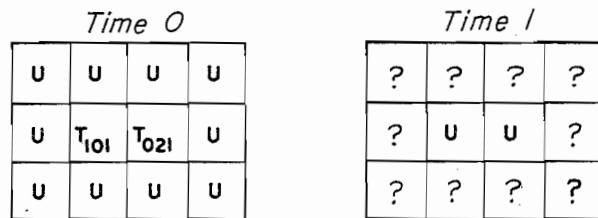
(b) Special and ordinary transmission states killing each other.
