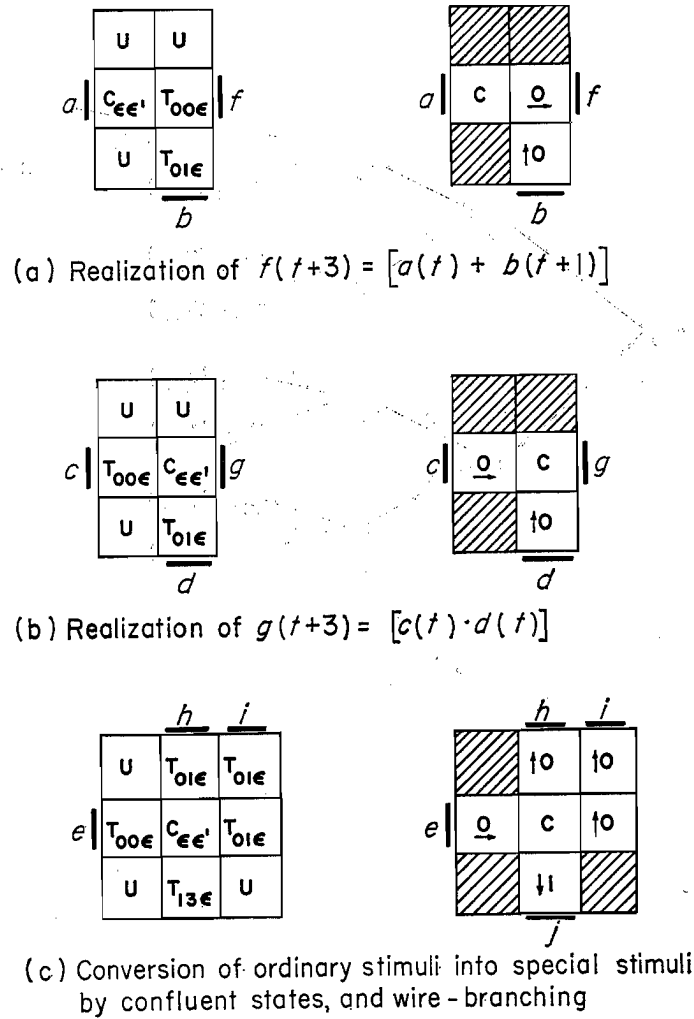
Fig. 11. Illustrations of transmission and confluent states
