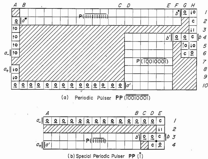
Fig. 17. Two periodic pulsers
