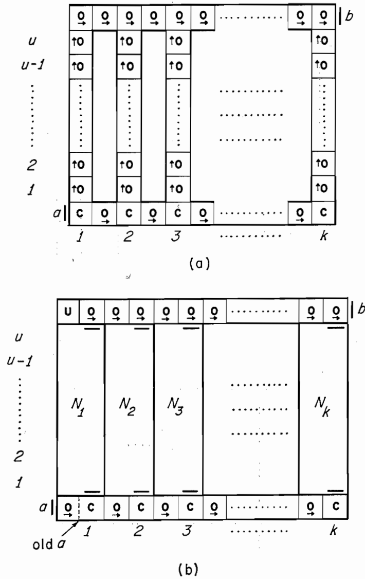
Fig. 16. Design of a pulser
