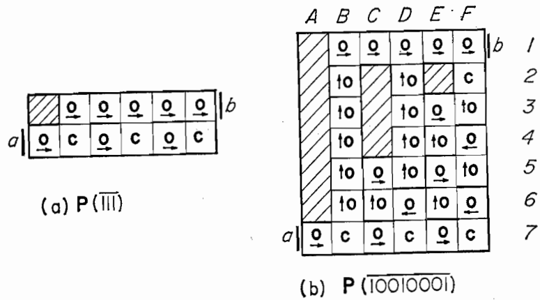
Fig. 15. Two pulsers
