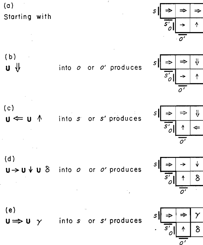
Fig. 47. Horizontal retreat of constructing arm with construction of \gamma and \delta
