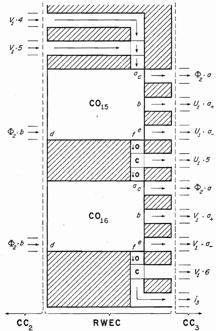
Fig. 41. Read-write-erase control RWEC . (f) Control organs for shortening the upper part of C_1 . (This completes Figure 41.)
