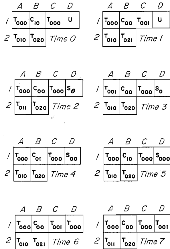
Fig. 12. Illustration of the direct process
