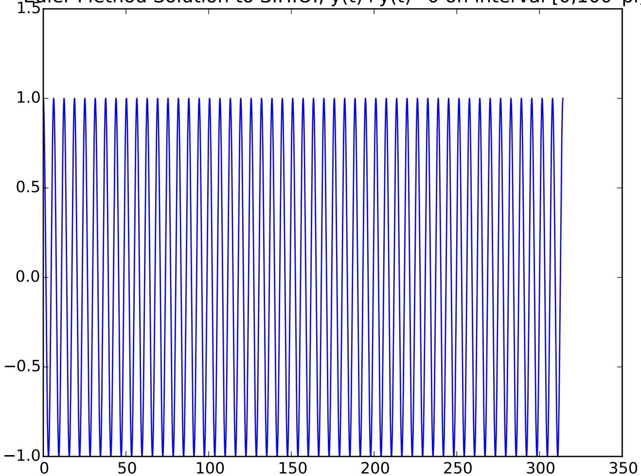
Euler Method Solution to S.H.O., y''+y(t)=0 on interval [0,100*\pi]
