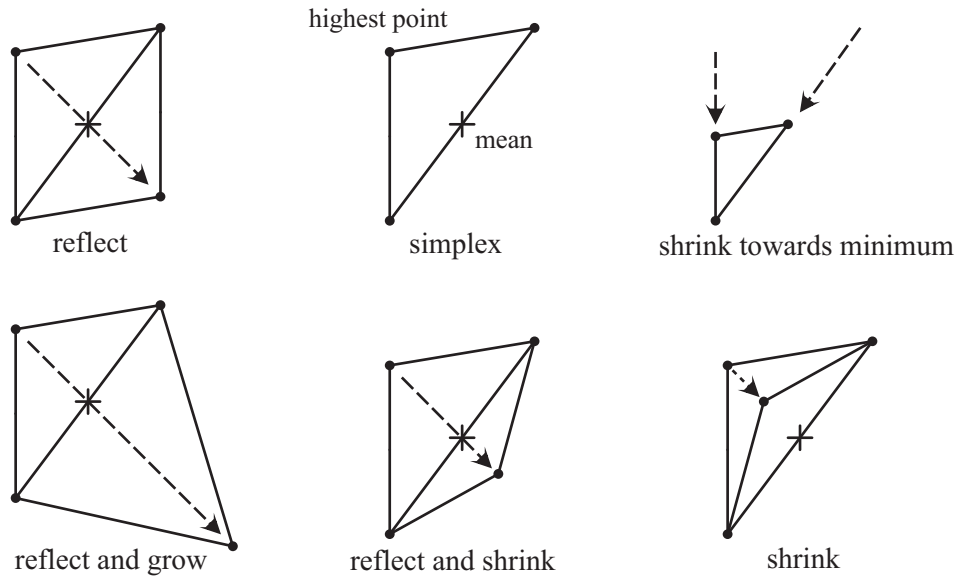
Figure 15.1. Downhill simplex update moves.
