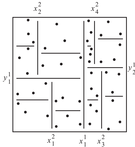
Figure 16.2. k -D tree binning in 2D.
