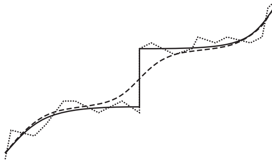
Figure 16.5. The problem with global regularization. A smoothness prior (dashed line) misses the discontinuity in the data (solid line); a maximum entropy prior (dotted) misses the smoothness.
