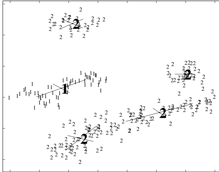
Figure 16.8. Cluster-weighted modeling with discrete output states. The small numbers are the events associated with each point; the large numbers are the most likely event associated with each cluster, and the lines are the cluster covariances.
