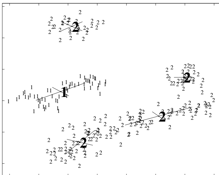
Figure 16.8. Cluster-weighted modeling with discrete output states. The small numbers are the events associated with each point; the large numbers are the most likely event associated with each cluster, and the lines are the cluster covariances.
