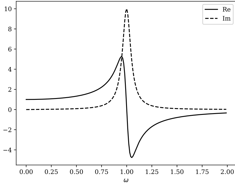
Figure 9.5. Anomalous dispersion
