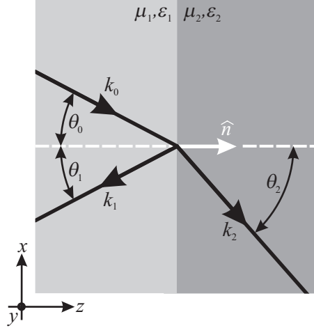
Figure 9.1. Reflection and refraction at an interface.
