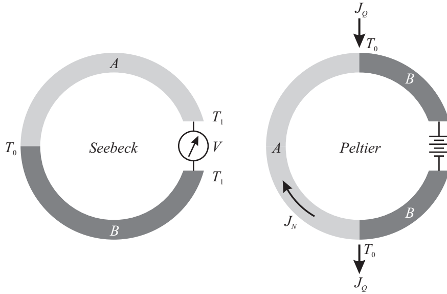
Figure 14.2. Thermoelectric effects.
