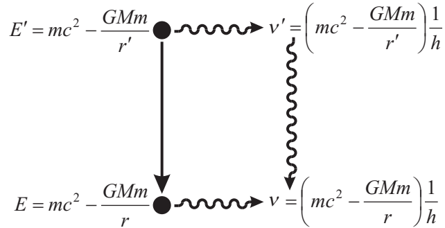
Figure 14.8. Gravitational red shift.
