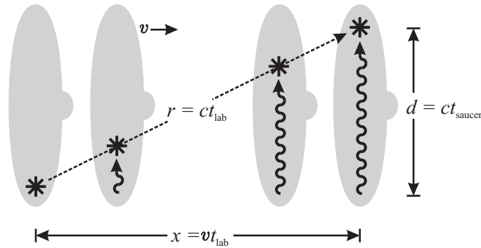
Figure 14.7. Time dilation.
