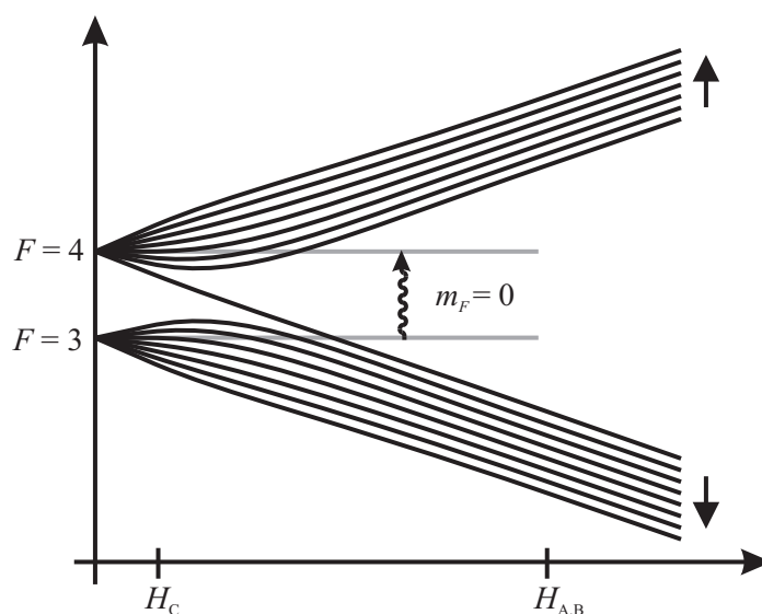
Figure 14.5. Cesium energy levels.
