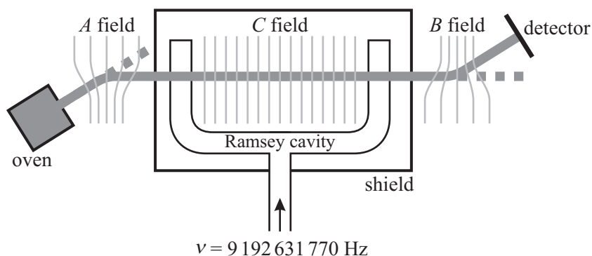
Figure 14.6. Cesium beam atomic clock.
