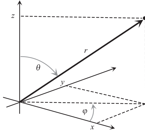
Figure 7.1. Rectangular, cylindrical, and spherical coordinate systems.
