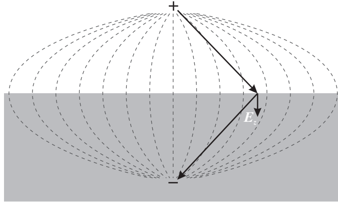
Figure 7.7. Image charge solution for the field of a charge above a ground plane.
