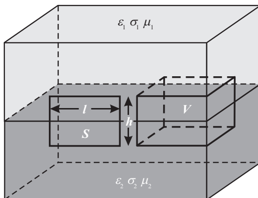
Figure 7.6. Loop and volume used for evaluating boundary conditions.
