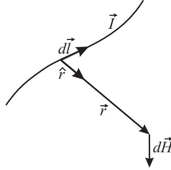
Figure 7.4. The magnetic field due to a differential current element.
