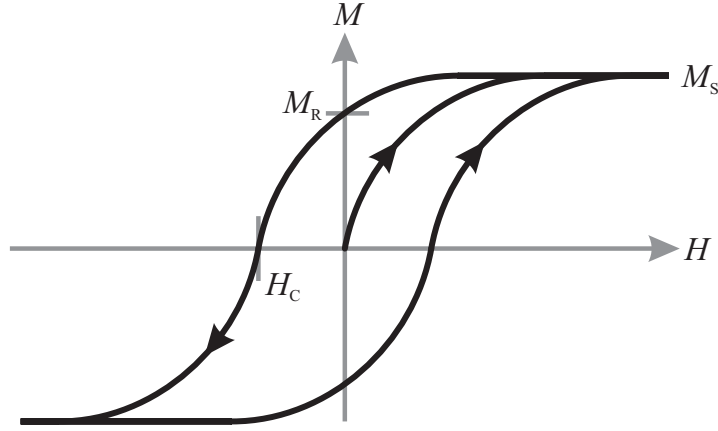
Figure 14.3. A hysteresis loop.
