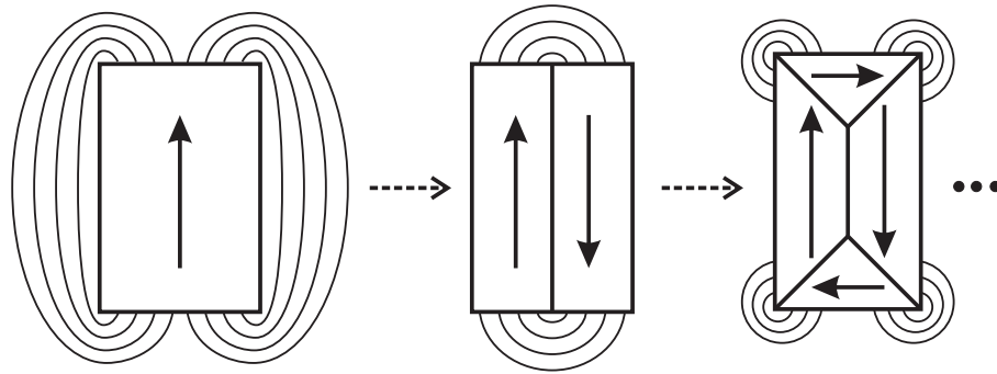
Figure 14.5. Magnetic domains reduce return flux energy.
