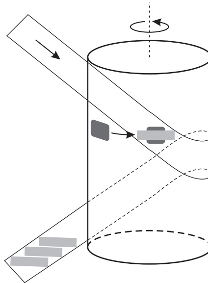
Figure 14.7. Tracks written by helical scan magnetic recording.
