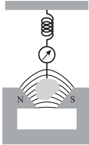
Figure 14.1. Measurement of permeability by an inhomogeneous field.
