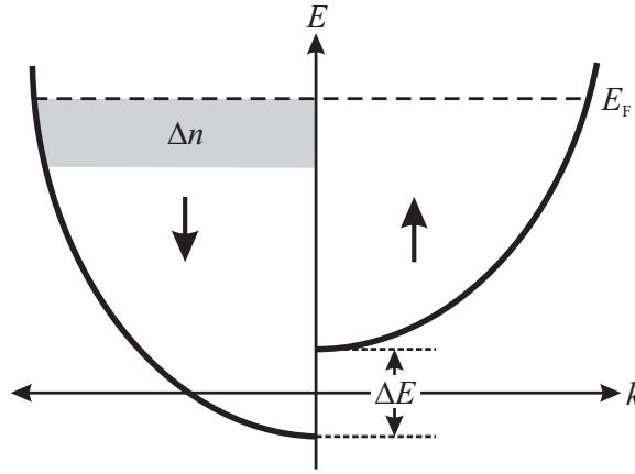
Figure 14.2. Spin band splitting in a field.
