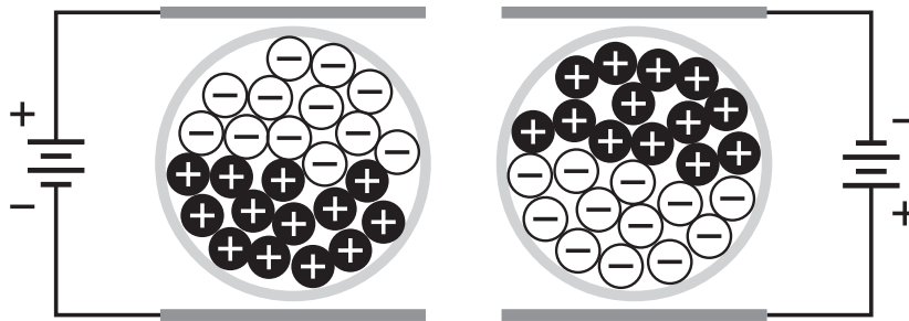
Figure 13.16. Microencapsulated electrophoretic electronic ink.
