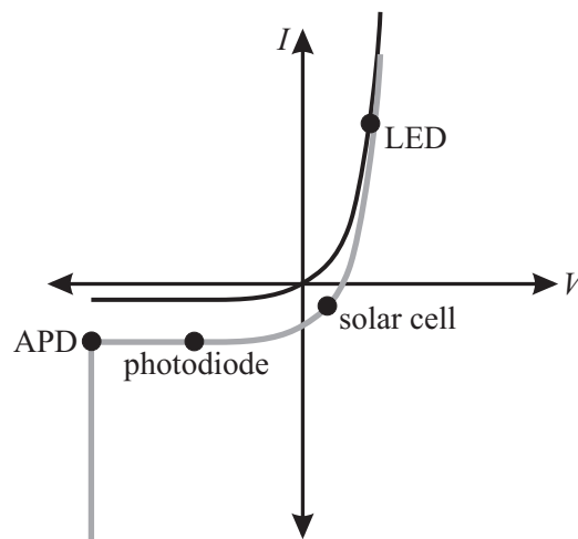
Figure 13.7. Biasing for a p-n junction.
