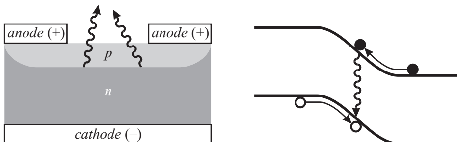
Figure 13.3. A Light-Emitting Diode.
