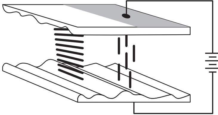
Figure 13.12. A twisted-nematic liquid crystal display.
