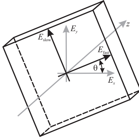
Figure 13.9. Axes in a birefringent crystal.
