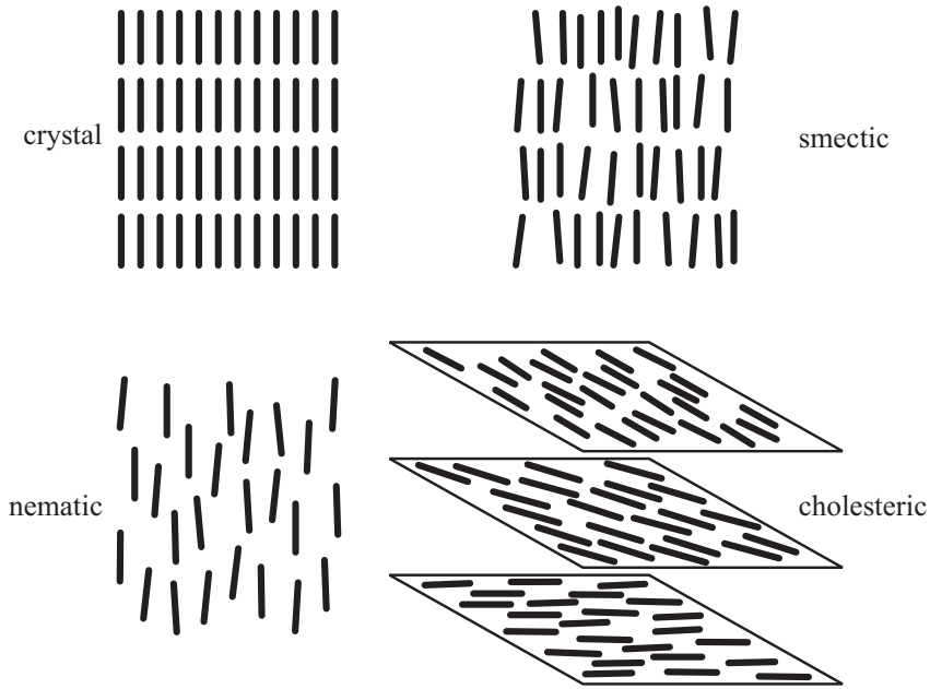
Figure 13.11. Liquid crystal ordering.
