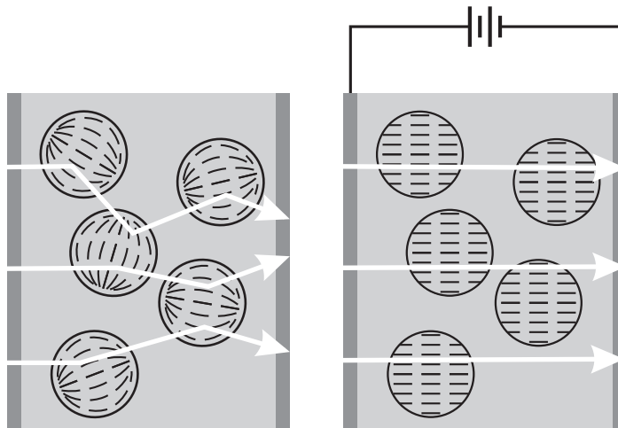
Figure 13.13. A polymer-dispersed liquid crystal panel.
