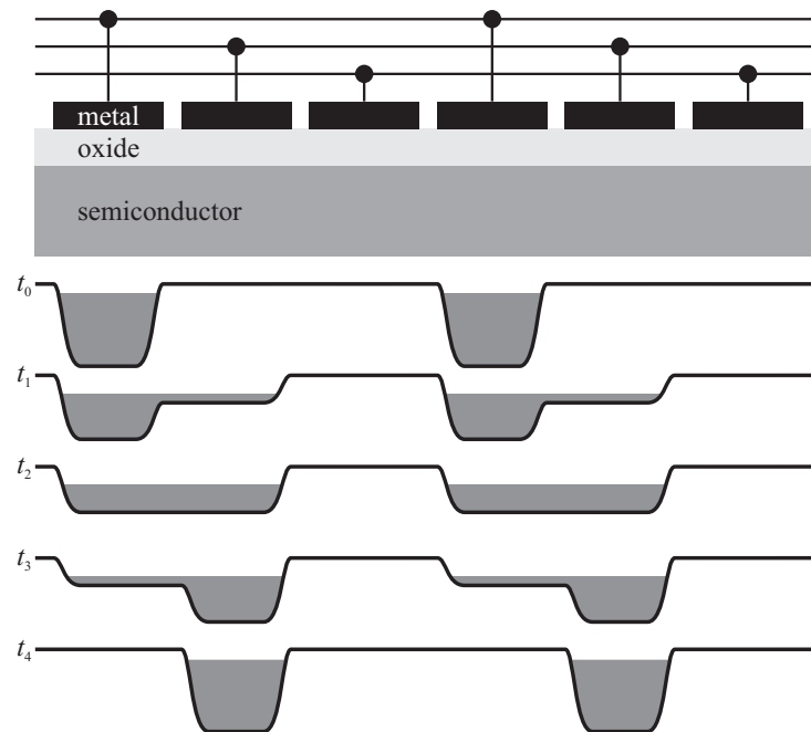
Figure 13.8. The operation of a CCD.
