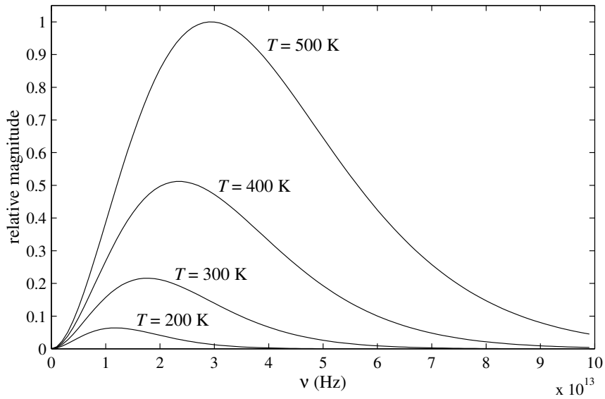
Figure 13.1. Planck's Law for thermal radiation.
