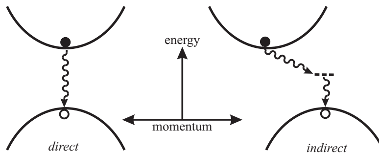
Figure 13.4. Semiconductor band gaps.
