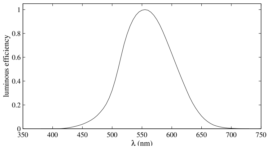
Figure 13.2. CIE luminosity function.
