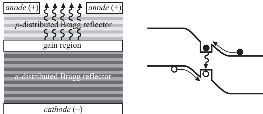
Figure 13.5. A Vertical-Cavity Surface-Emitting Laser.
