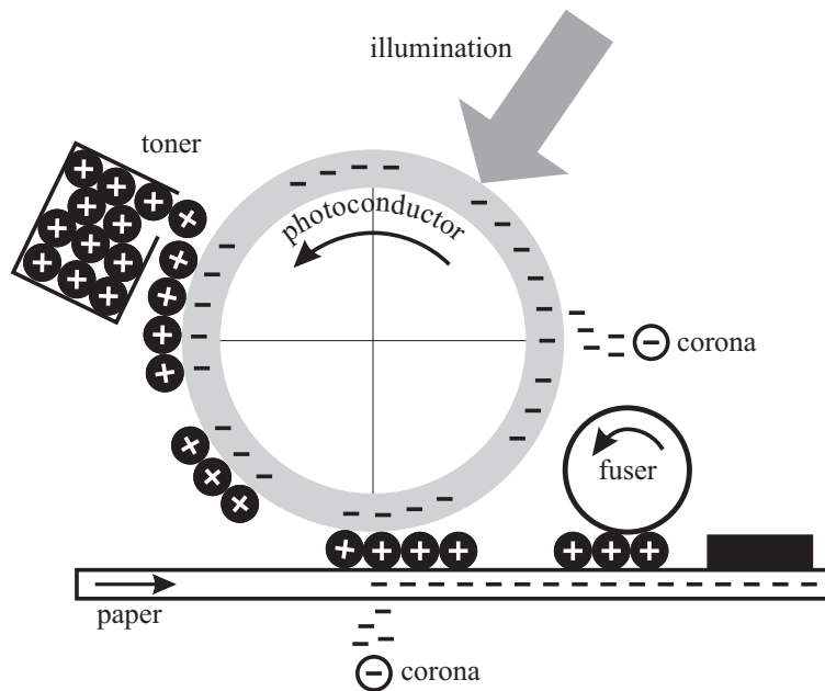
Figure 13.15. Electrophotography.
