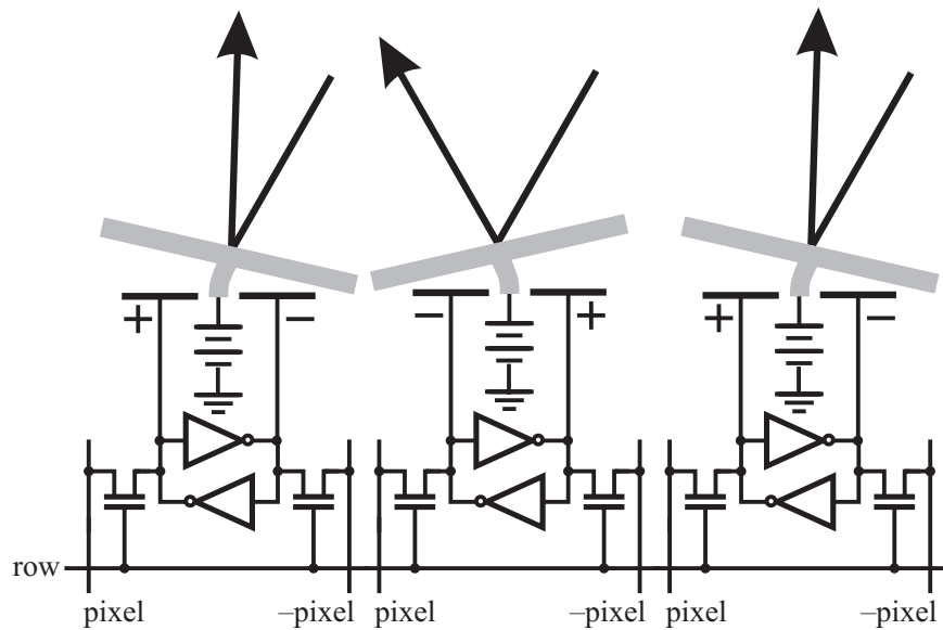
Figure 13.14. A Digital Micromirror Device.
