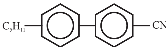
Figure 13.10. The liquid crystal 5CB.
