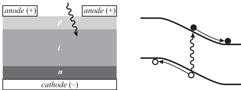
Figure 13.6. A p-i-n photodiode.
