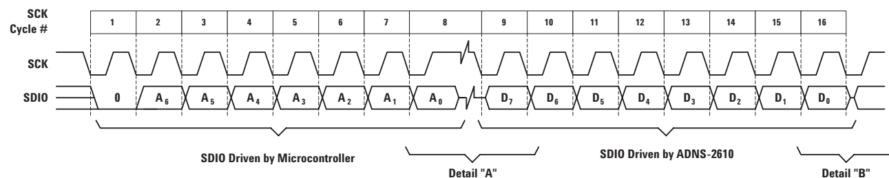
Figure 21. Read operation.
