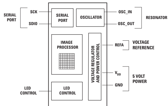
Figure 6. Block diagram of ADNS-2610 optical mouse sensor.
