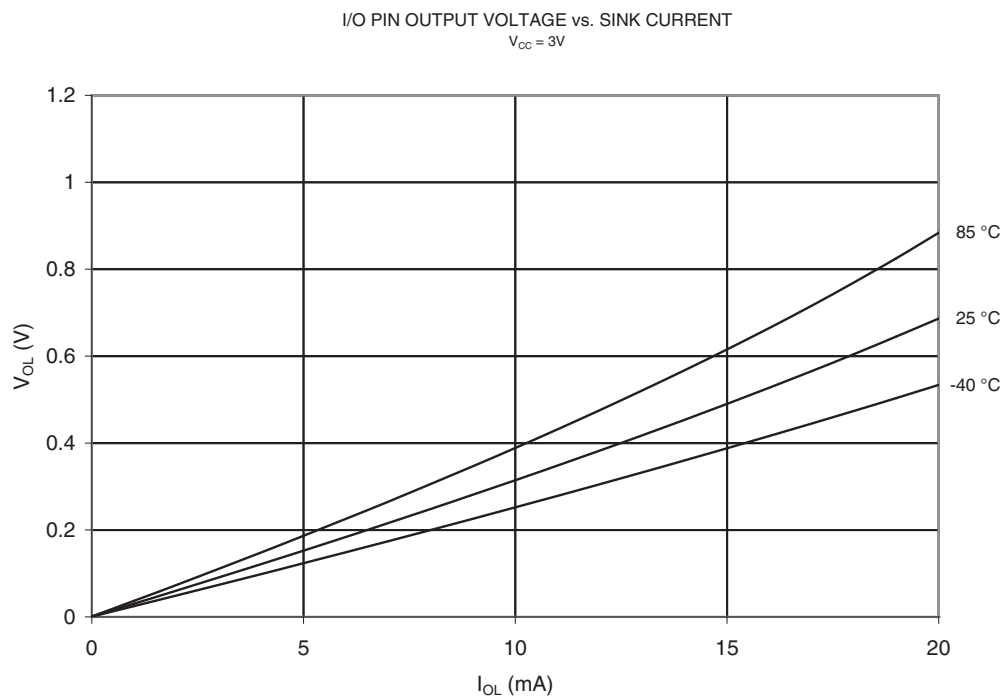
Figure 21-82. V_{OL} : Output Voltage vs. Sink Current (I/O Pin, V_{CC} = 3V )
