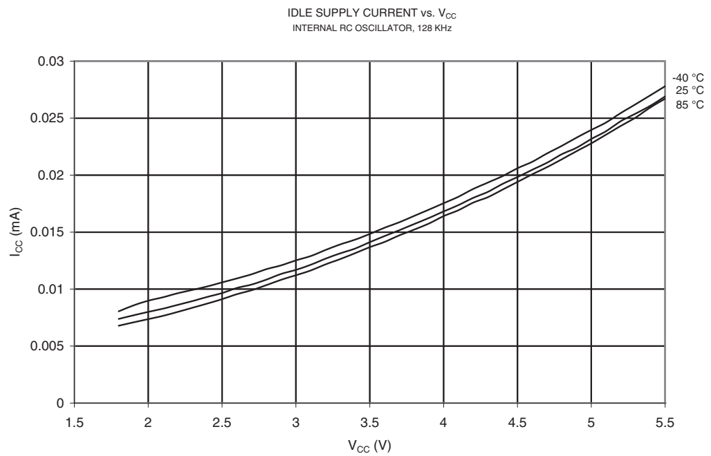
Figure 21-64. Idle Supply Current vs. V_{CC} (Internal RC Oscillator, 128 kHz)
