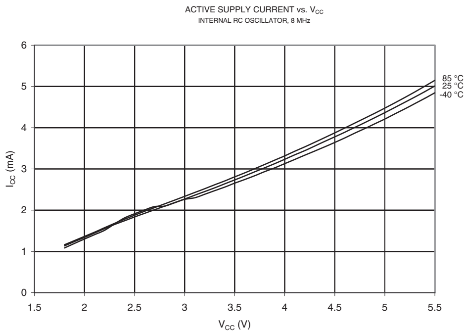
Figure 21-57. Active Supply Current vs. V_{CC} (Internal RC Oscillator, 8 MHz)
