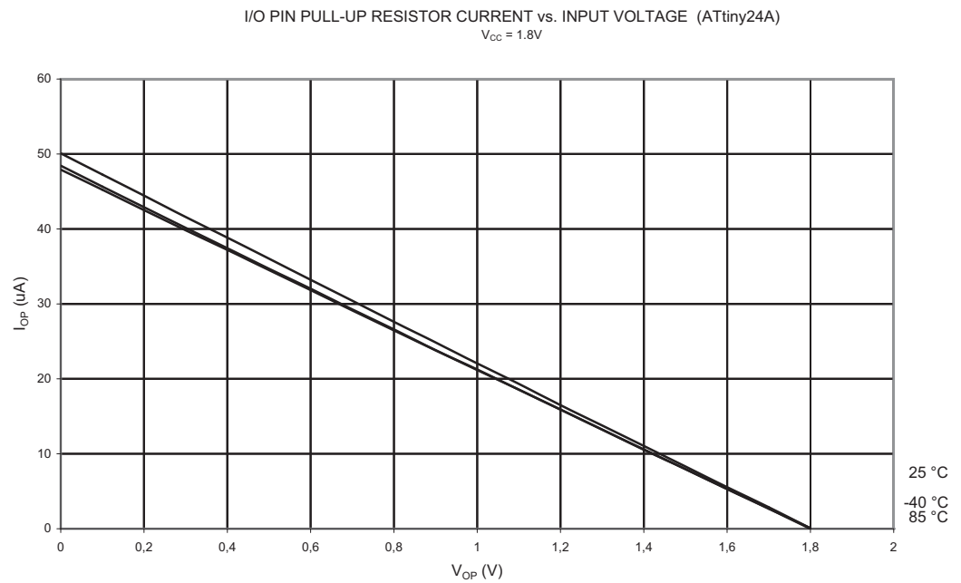
Figure 21-21. Pull-up Resistor Current vs. Input Voltage (I/O Pin, V_{CC} = 1.8V )
