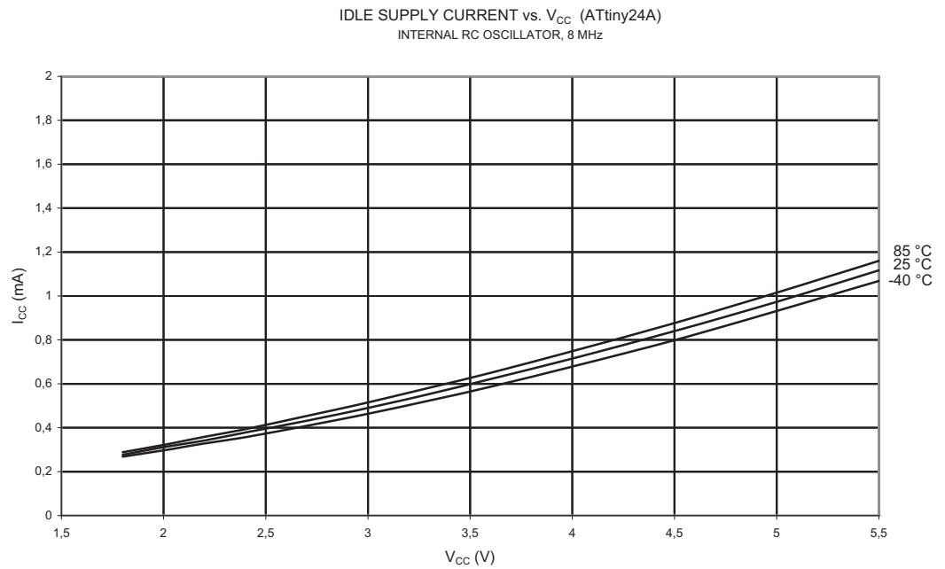
Figure 21-8. Idle Supply Current vs. V_{CC} (Internal RC Oscillator, 8 MHz)
