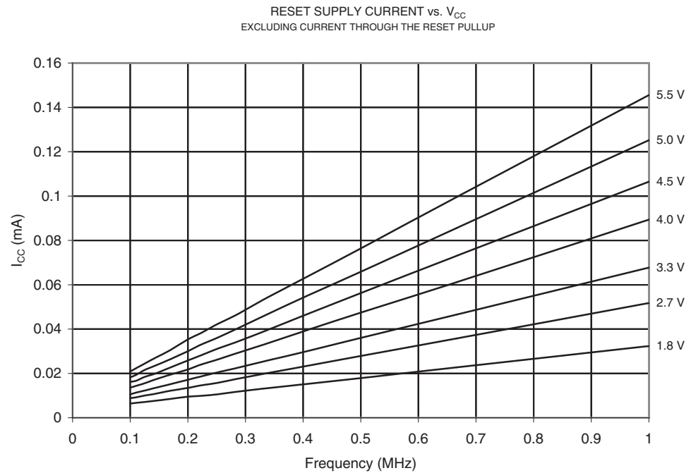
Figure 21-67. Reset Supply Current vs. V_{CC} (0.1 - 1.0 MHz, excluding Current Through the Reset Pull-up)
