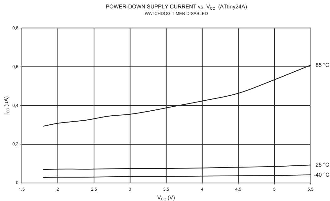
Figure 21-11. Power-down Supply Current vs. V_{CC} (Watchdog Timer Disabled)
