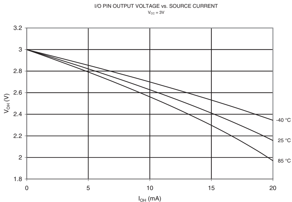
Figure 21-84. V_{OH} : Output Voltage vs. Source Current (I/O Pin, V_{CC} = 3V )
