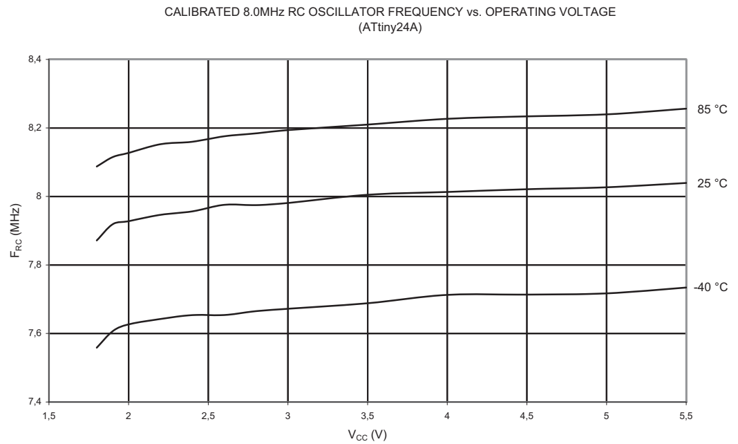
Figure 21-52. Calibrated 8 MHz RC Oscillator Frequency vs. V_{CC}
