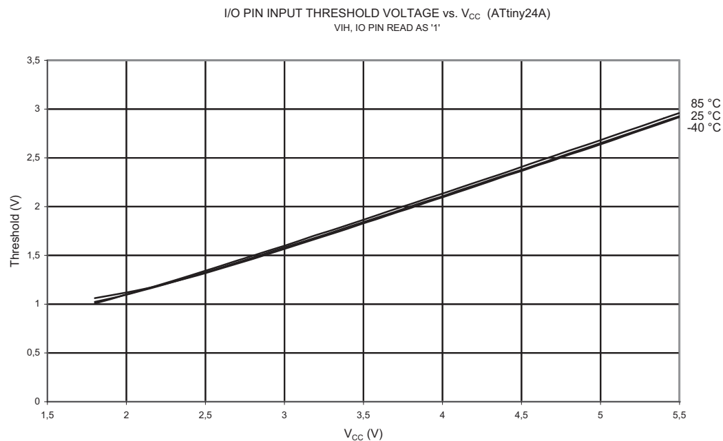
Figure 21-35. V_{IH} : Input Threshold Voltage vs. V_{CC} (IO Pin, Read as '1')
