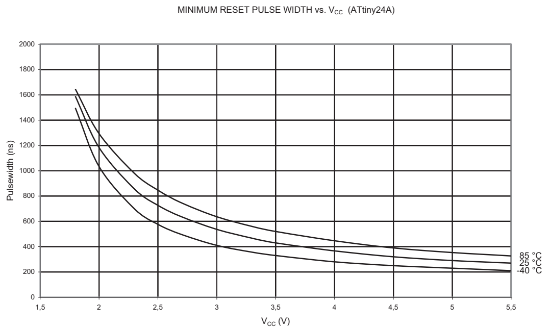
Figure 21-49. Minimum Reset Pulse Width vs. V_{CC}
