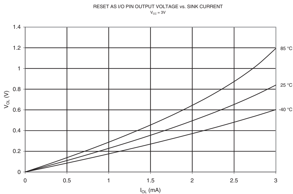
Figure 21-86. V_{OL} : Output Voltage vs. Sink Current (Reset Pin as I/O, V_{CC} = 3V )
