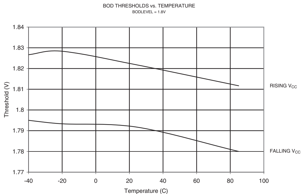
Figure 21-98. BOD Threshold vs. Temperature (BODLEVEL is 1.8V)
