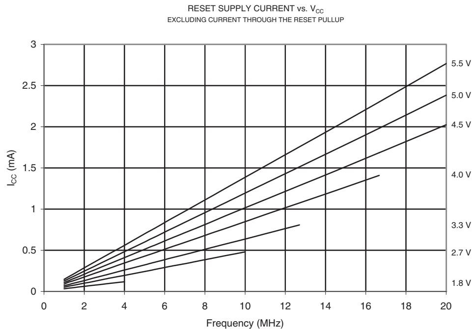
Figure 21-68. Reset Supply Current vs. V_{CC} (1 - 20 MHz, Excluding Current Through the Reset Pull-up)
