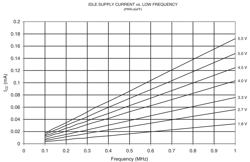
Figure 21-60. Idle Supply Current vs. Low Frequency (0.1 - 1.0 MHz)
