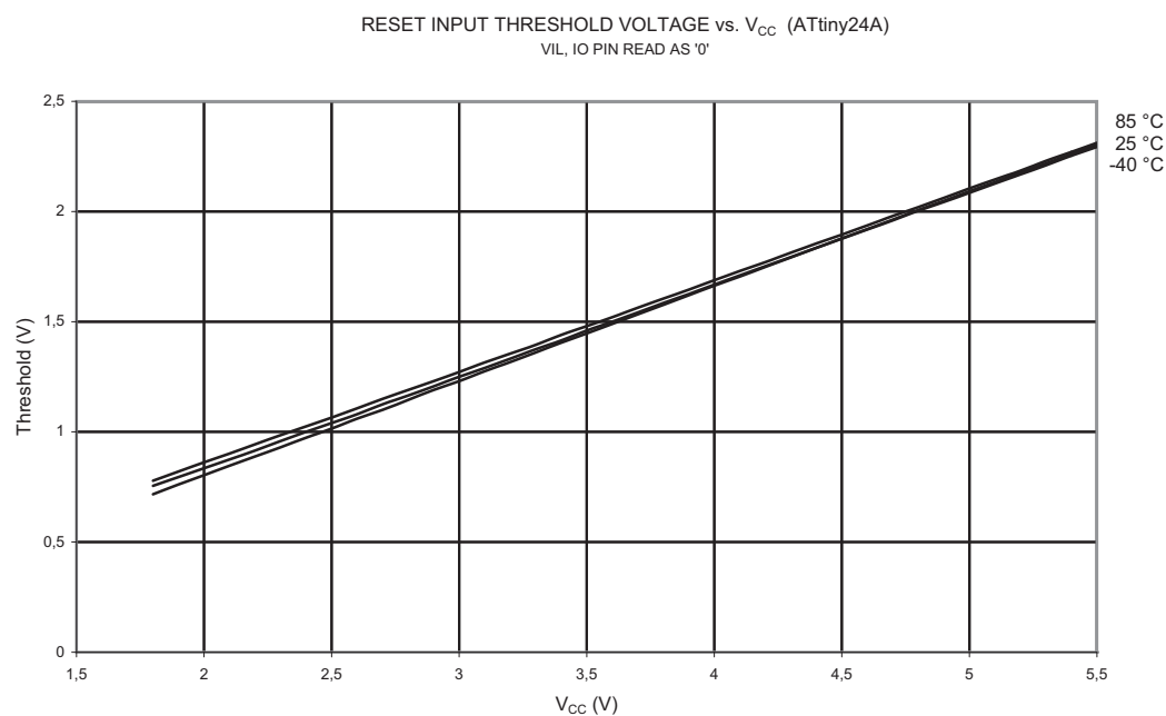
Figure 21-47. V_{IL} : Input Threshold Voltage vs. V_{CC} (Reset Pin, Read as '0')
