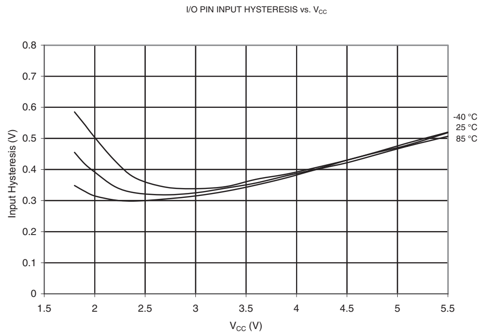
Figure 21-92. V_{IH}-V_{IL} : Input Hysteresis vs. V_{CC} (I/O Pin)
