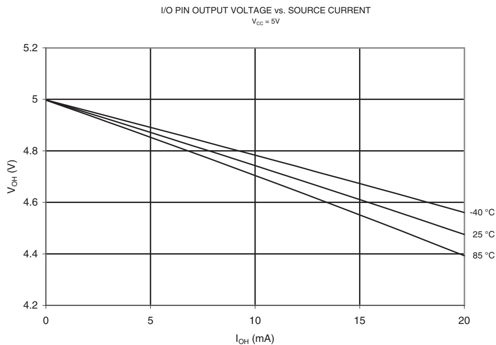
Figure 21-85. V_{OH} : Output Voltage vs. Source Current (I/O Pin, V_{CC} = 5V )
