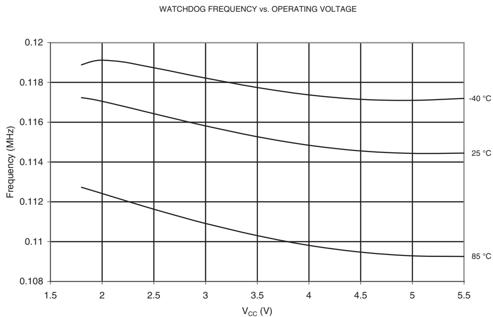
Figure 21-105. Watchdog Oscillator Frequency vs. V_{CC}
