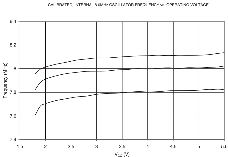
Figure 21-107. Calibrated 8 MHz RC Oscillator Frequency vs. V_{CC}
