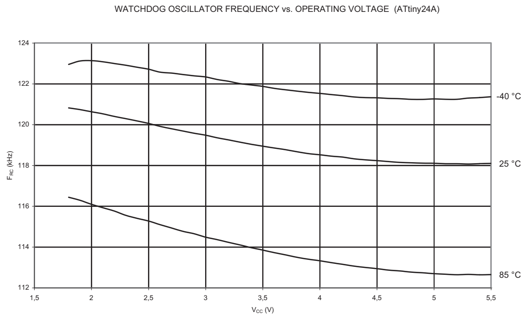
Figure 21-50. Watchdog Oscillator Frequency vs. V_{CC}
