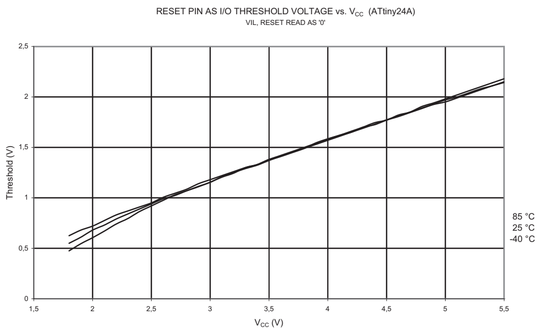
Figure 21-39. V_{IL} : Input Threshold Voltage vs. V_{CC} (Reset Pin as I/O, Read as '0')
