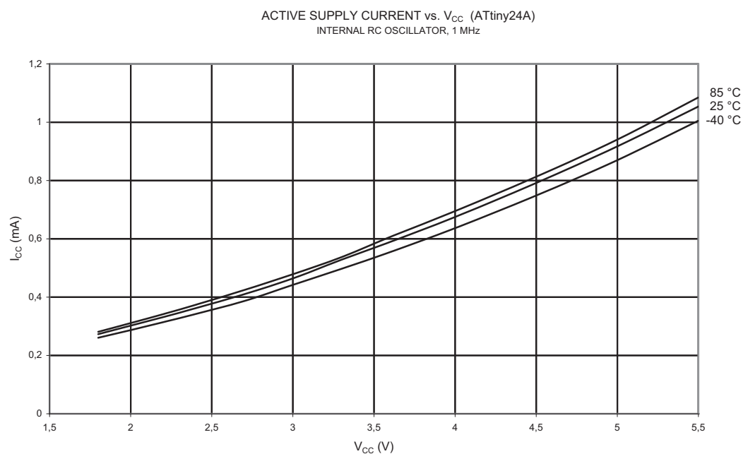
Figure 21-4. Active Supply Current vs. V_{CC} (Internal RC Oscillator, 1 MHz)
