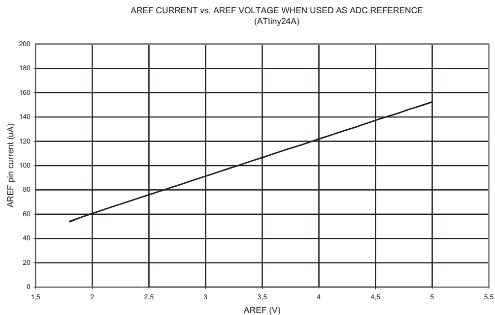
Figure 21-16. AREF External Reference Current vs. V_{CC}
