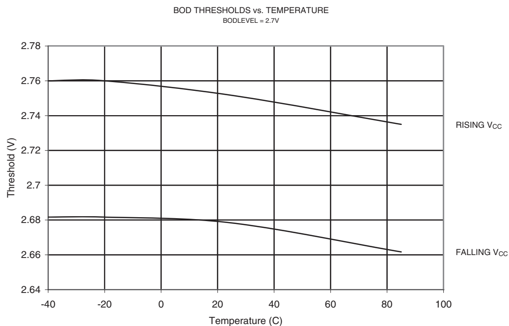
Figure 21-97. BOD Threshold vs. Temperature (BODLEVEL is 2.7V)
