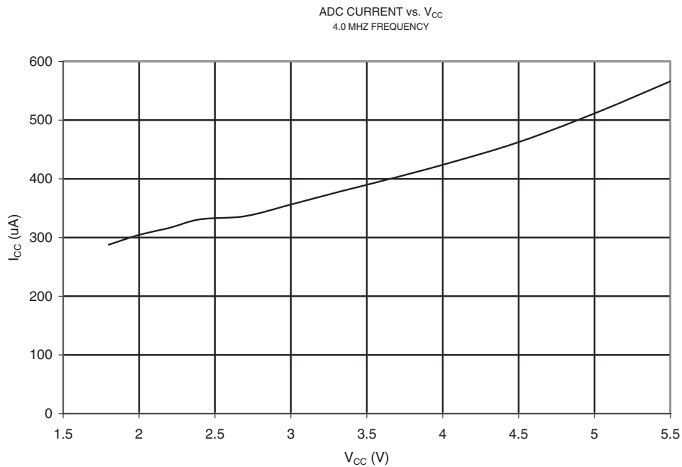
Figure 21-69. ADC Current vs. V_{CC}
