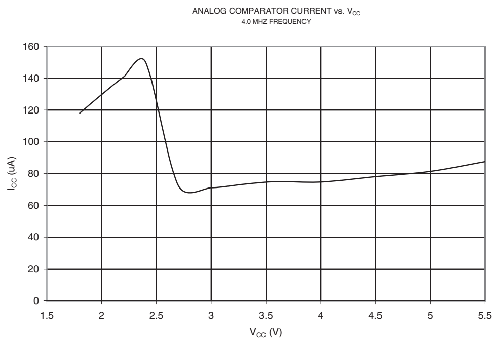
Figure 21-71. Analog Comparator Current vs. V_{CC}
