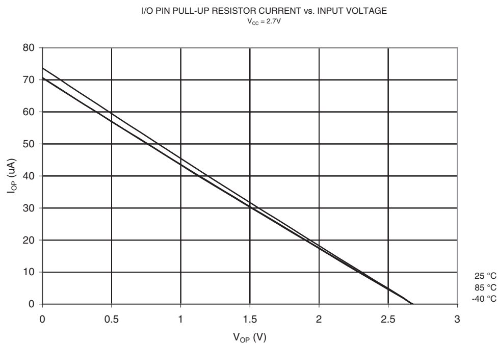
Figure 21-77. Pull-up Resistor Current vs. Input Voltage (I/O Pin, V_{CC} = 2.7V )
