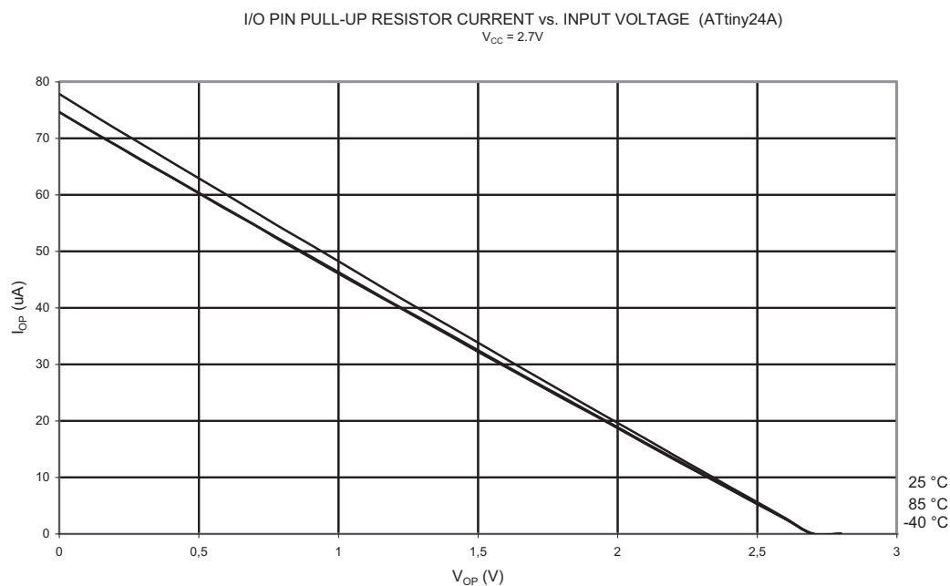
Figure 21-22. Pull-up Resistor Current vs. Input Voltage (I/O Pin, V_{CC} = 2.7V )
