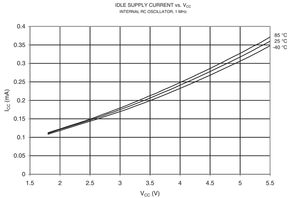
Figure 21-63. Idle Supply Current vs. V_{CC} (Internal RC Oscillator, 1 MHz)
