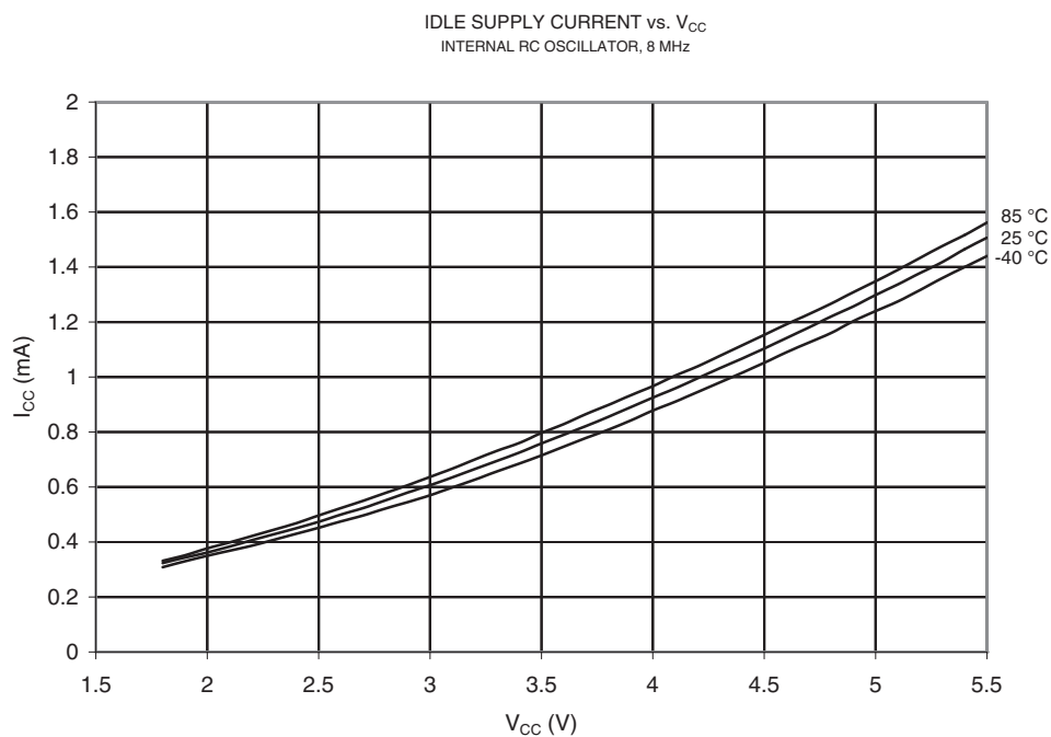
Figure 21-62. Idle Supply Current vs. V_{CC} (Internal RC Oscillator, 8 MHz)
