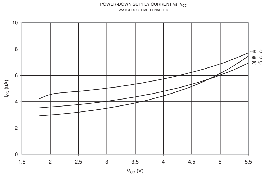
Figure 21-66. Power-down Supply Current vs. V_{CC} (Watchdog Timer Enabled)
