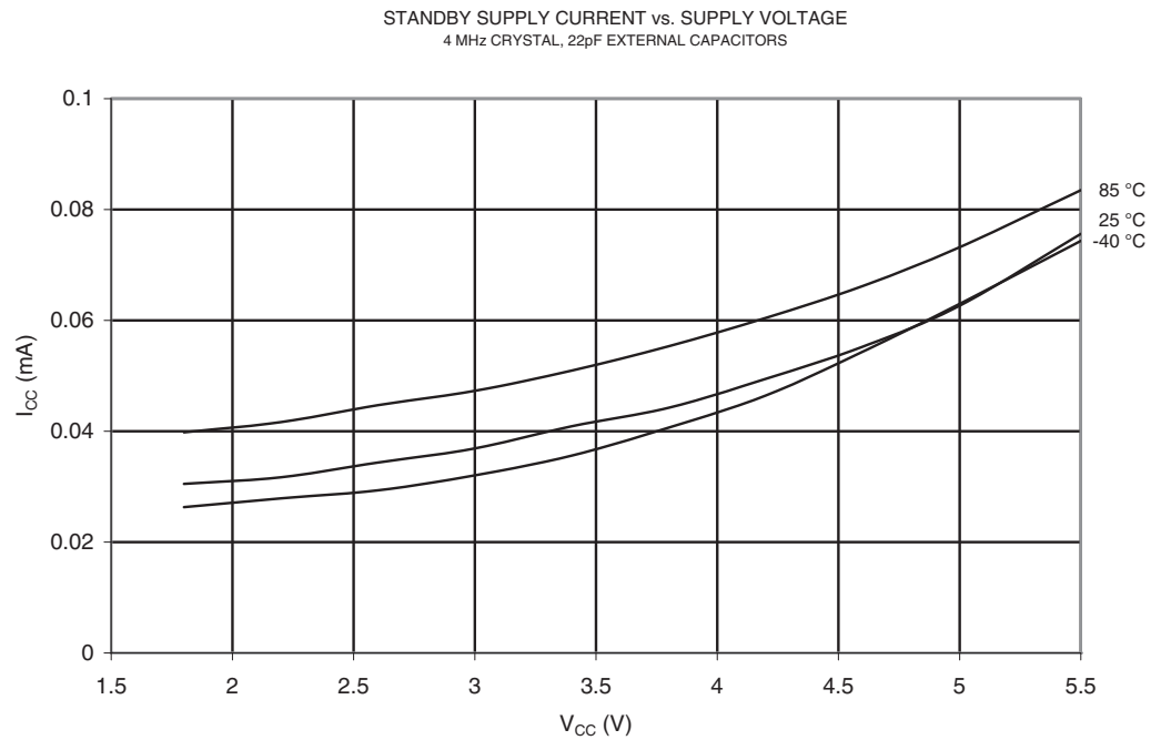
Figure 21-75. Standby Supply Current vs. V_{CC} (4 MHz External Crystal, External Capacitors, Watchdog Timer Disabled)
