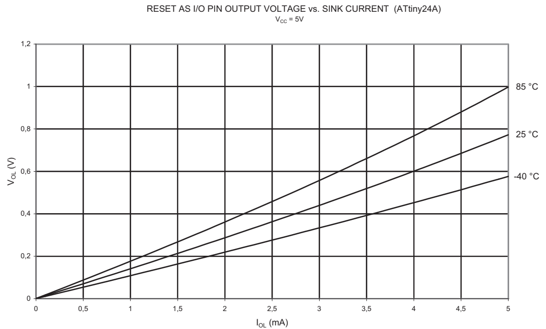
Figure 21-32. V_{OL} : Output Voltage vs. Sink Current (Reset Pin as I/O, V_{CC} = 5V )
