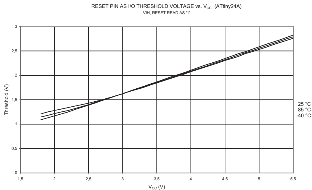
Figure 21-38. V_{IH} : Input Threshold Voltage vs. V_{CC} (Reset Pin as I/O, Read as '1')
