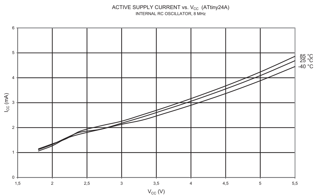
Figure 21-3. Active Supply Current vs. V_{CC} (Internal RC Oscillator, 8 MHz)
