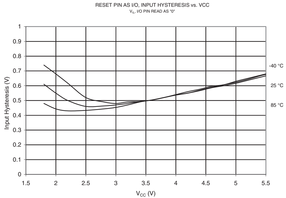
Figure 21-95. V_{IH} - V_{IL} : Input Hysteresis vs. V_{CC} (Reset Pin as I/O)
