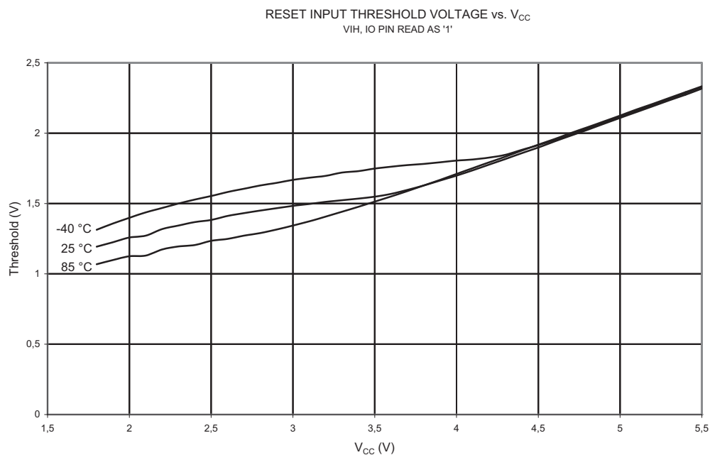
Figure 21-101. V_{IH} : Input Threshold Voltage vs. V_{CC} (Reset Pin, Read as '1')
