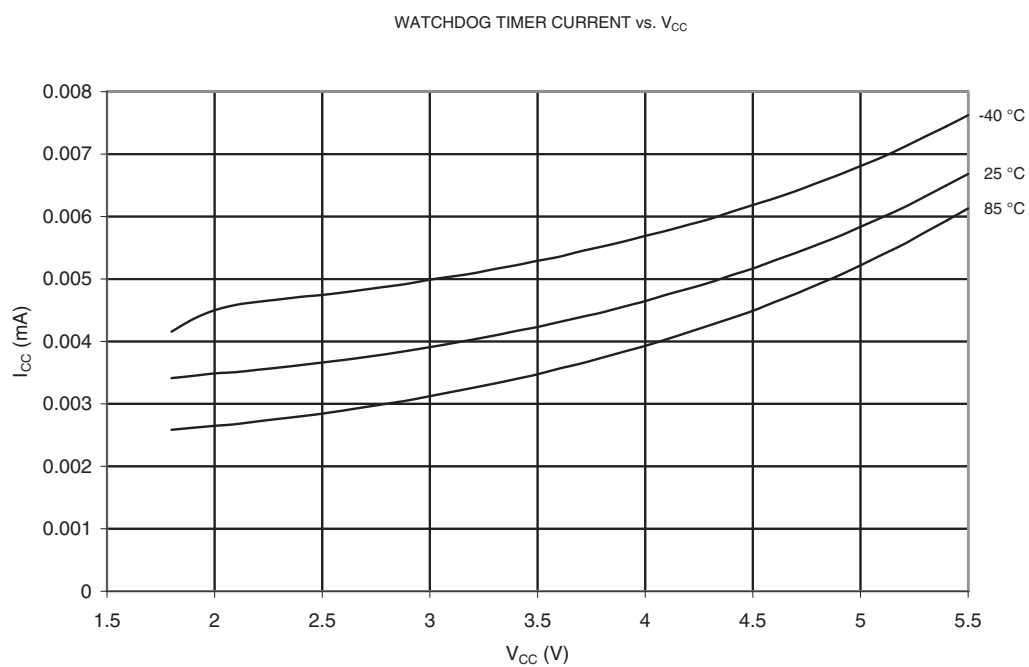
Figure 21-74. Watchdog Timer Current vs. V_{CC}
