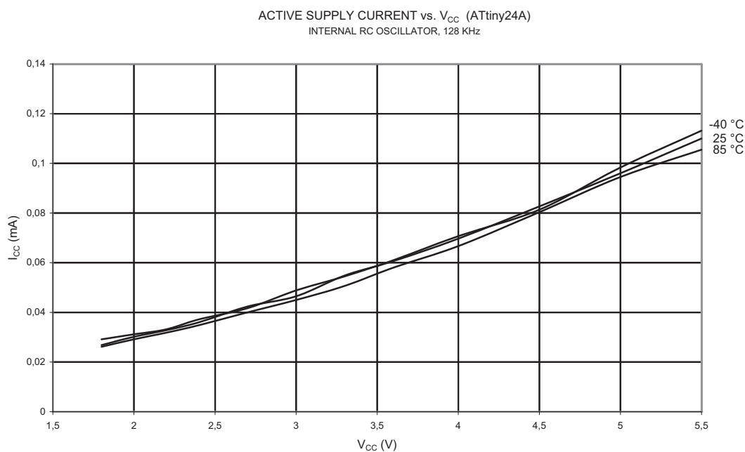
Figure 21-5. Active Supply Current vs. V_{CC} (Internal RC Oscillator, 128 kHz)
