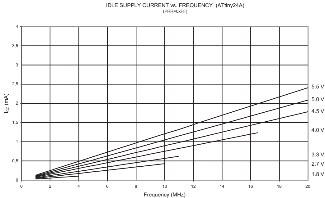
Figure 21-7. Idle Supply Current vs. Frequency (1 - 20 MHz)
