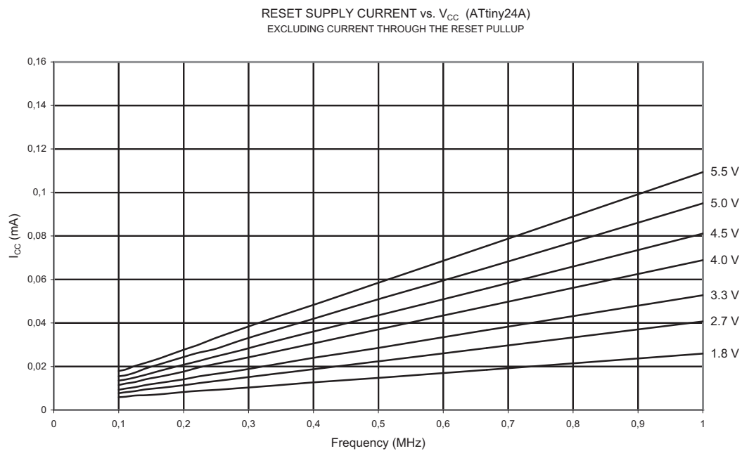
Figure 21-13. Reset Supply Current vs. V_{CC} (0.1 - 1.0 MHz, excluding Current Through the Reset Pull-up)
