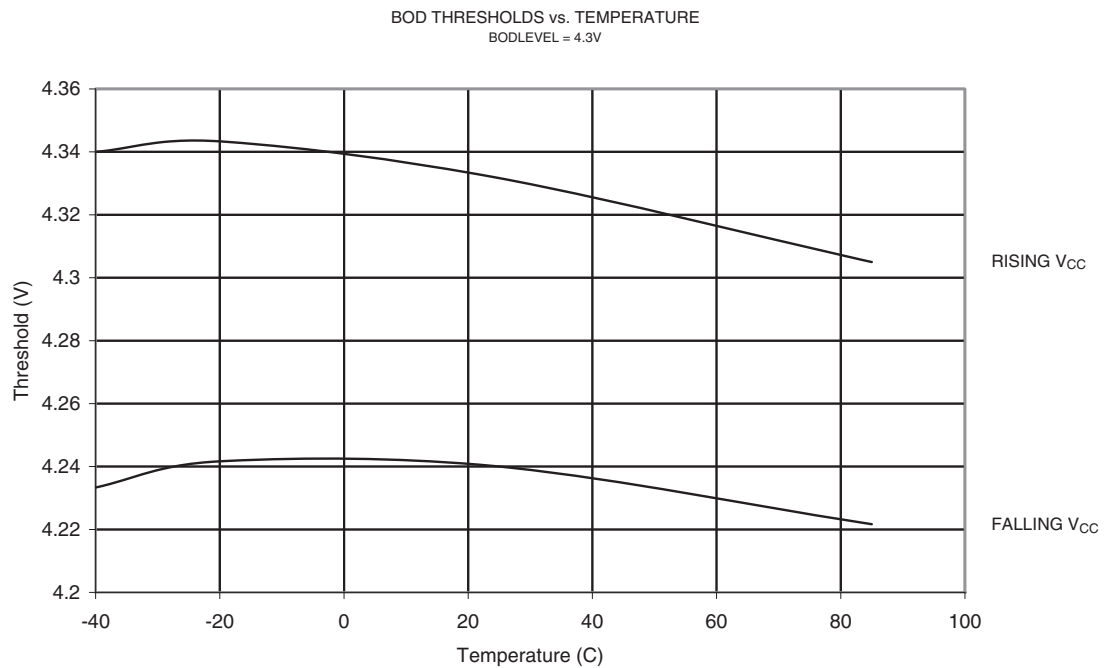
Figure 21-96. BOD Threshold vs. Temperature (BODLEVEL is 4.3V)
