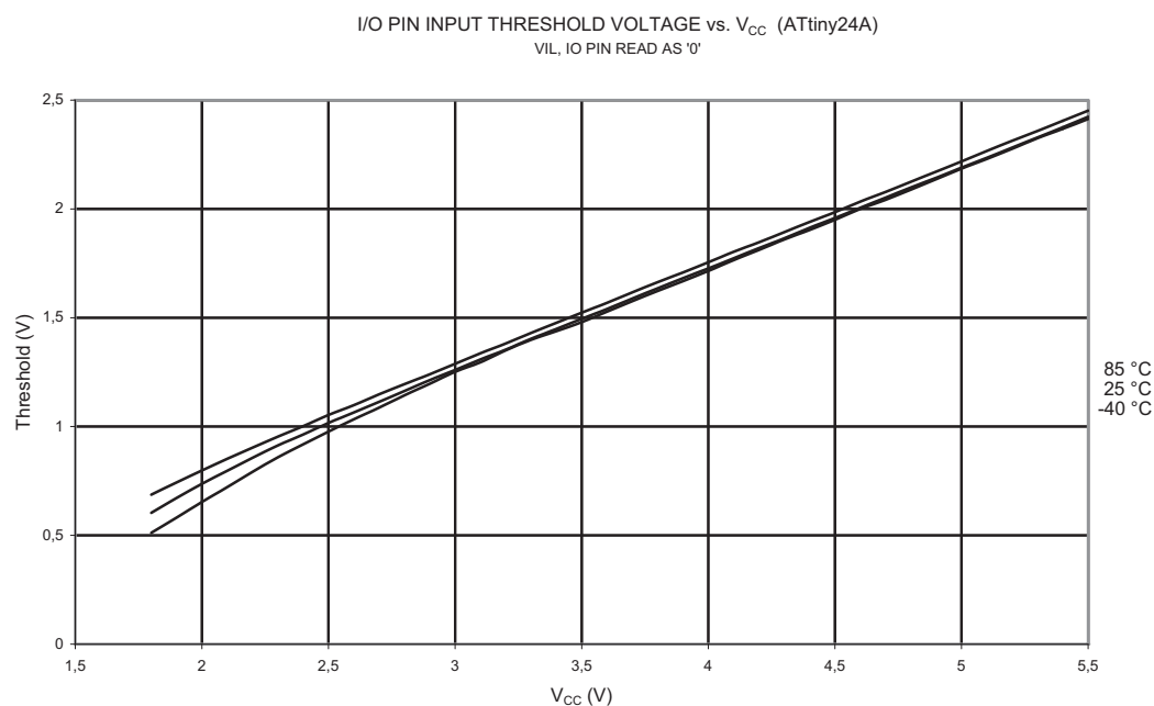
Figure 21-36. V_{IL} : Input Threshold Voltage vs. V_{CC} (I/O Pin, Read as '0')
