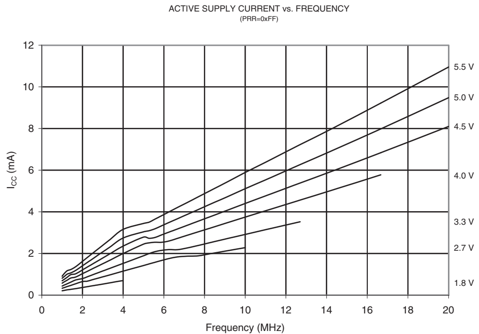
Figure 21-56. Active Supply Current vs. frequency (1 - 20 MHz)
