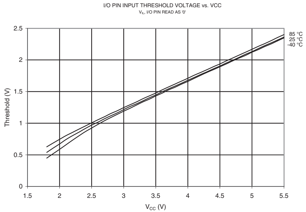
Figure 21-91. V_{IL} : Input Threshold Voltage vs. V_{CC} (I/O Pin, Read as '0')
