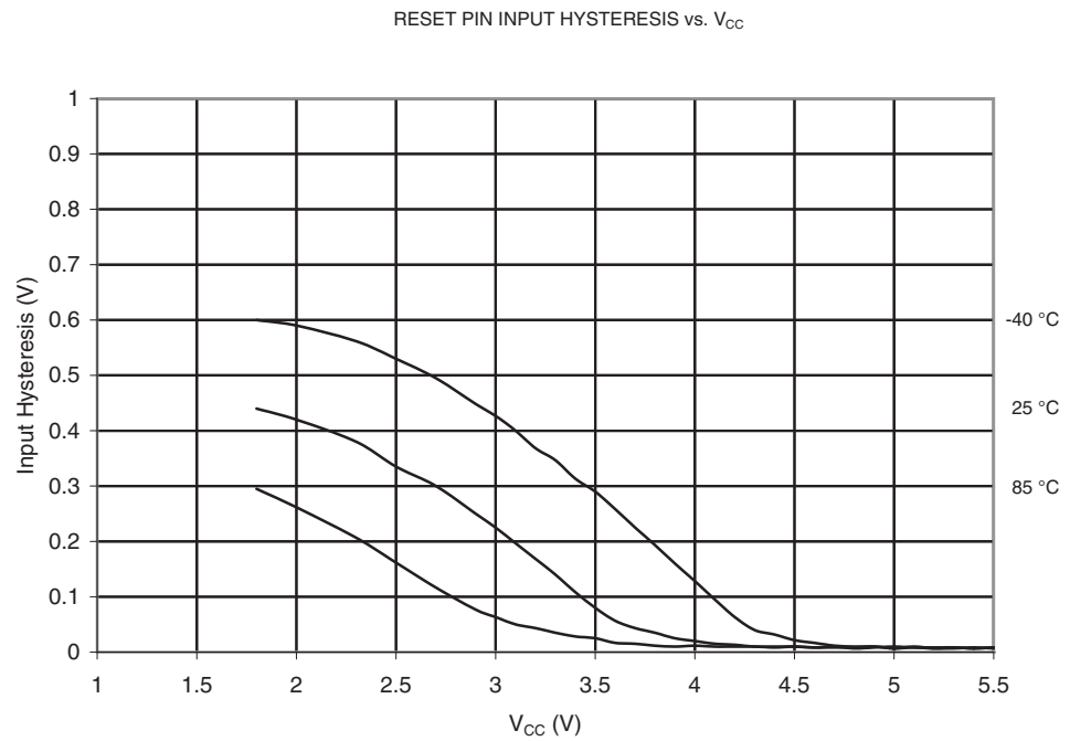
Figure 21-103. V_{IH} - V_{IL} : Input Hysteresis vs. V_{CC} (Reset Pin)
