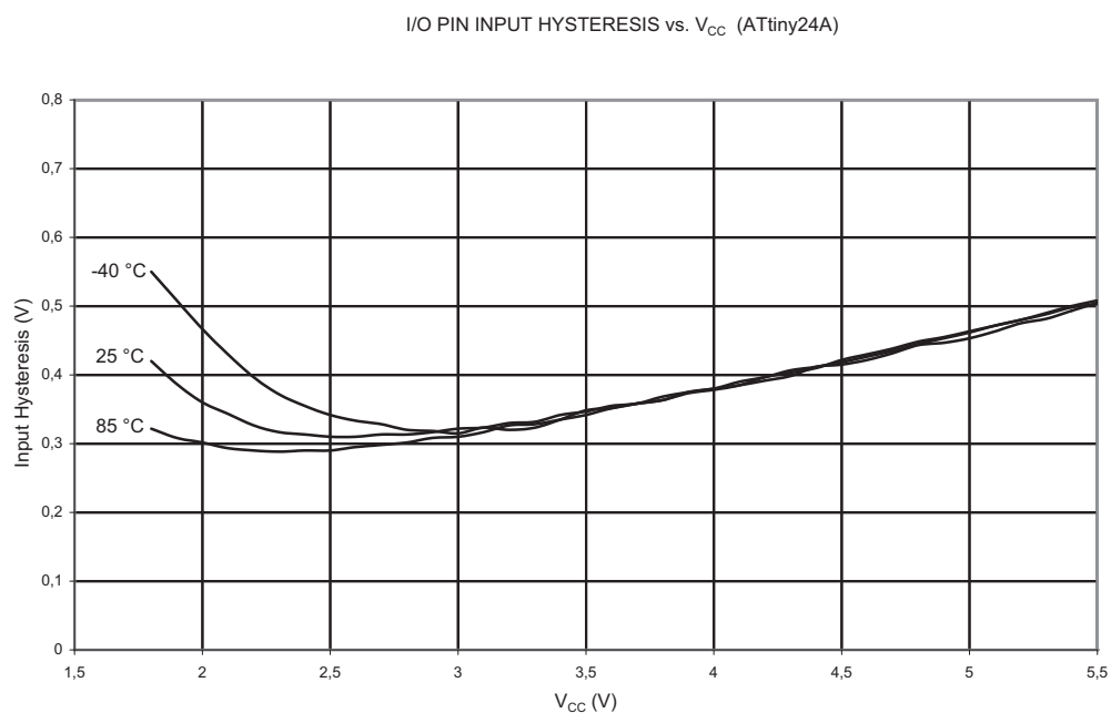
Figure 21-37. V_{IH}-V_{IL} : Input Hysteresis vs. V_{CC} (I/O Pin)
