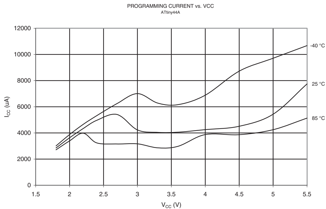
Figure 21-72. Programming Current vs. V_{CC} (ATtiny44A)
