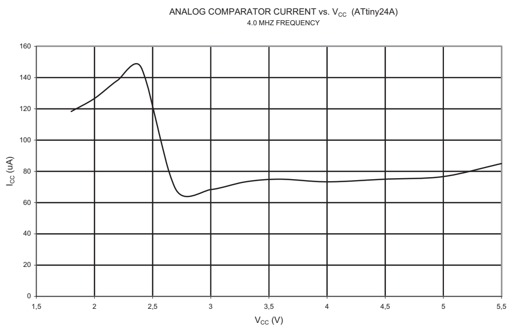
Figure 21-17. Analog Comparator Current vs. V_{CC}
