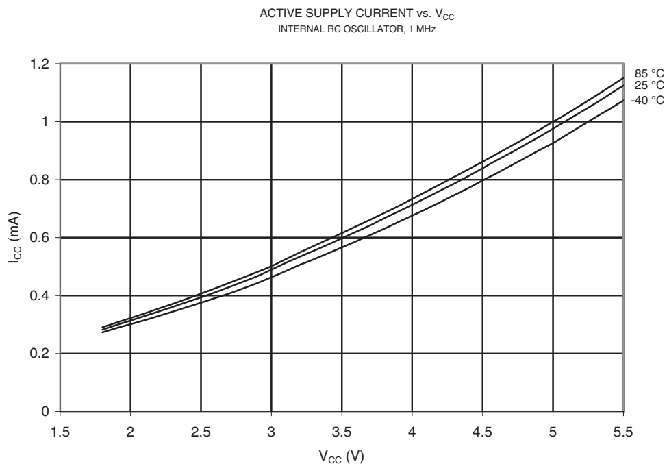
Figure 21-58. Active Supply Current vs. V_{CC} (Internal RC Oscillator, 1 MHz)
