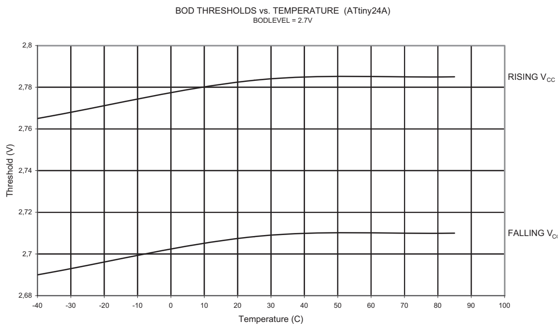
Figure 21-42. BOD Threshold vs. Temperature (BODLEVEL is 2.7V)
