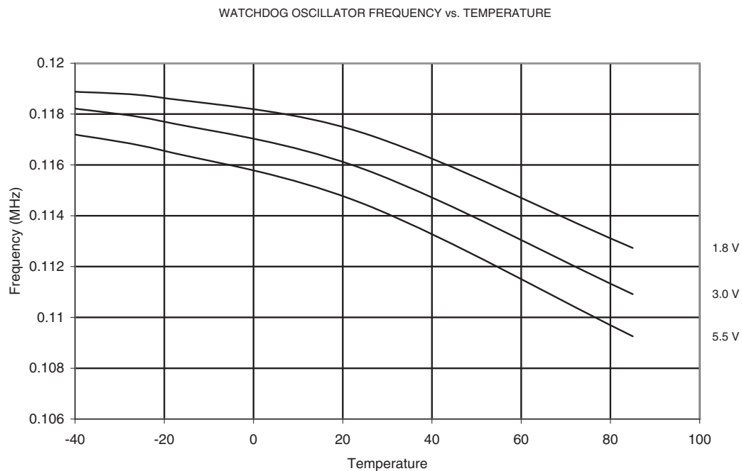
Figure 21-106. Watchdog Oscillator Frequency vs. Temperature
