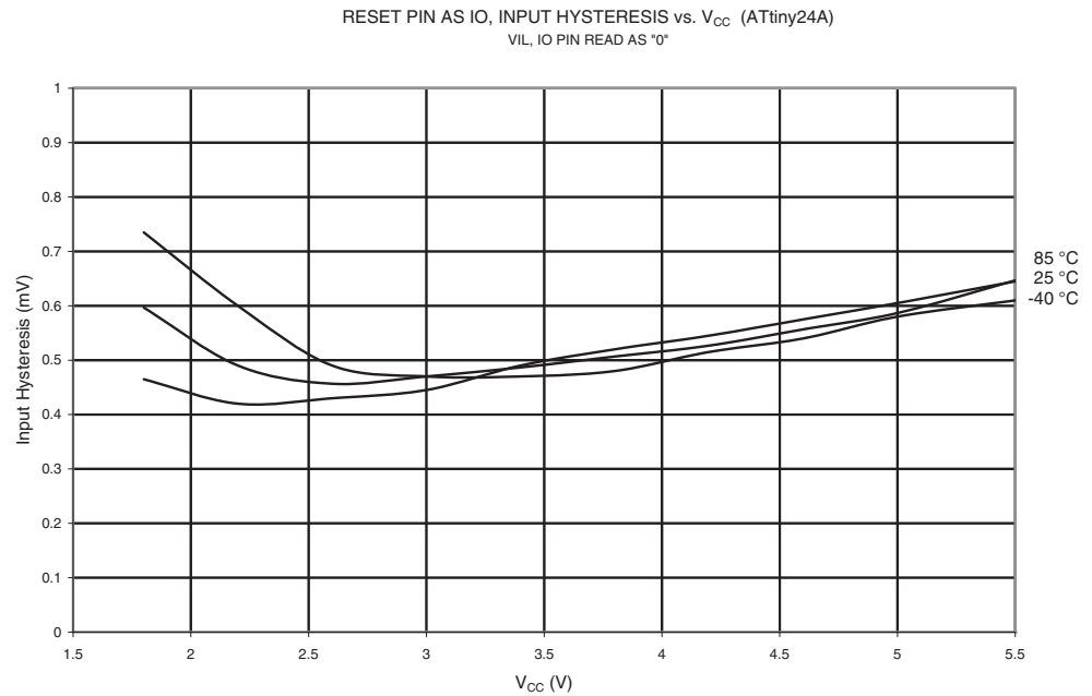
Figure 21-40. V_{IH}-V_{IL} : Input Hysteresis vs. V_{CC} (Reset Pin as I/O)
