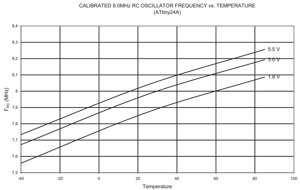
Figure 21-53. Calibrated 8 MHz RC oscillator Frequency vs. Temperature
