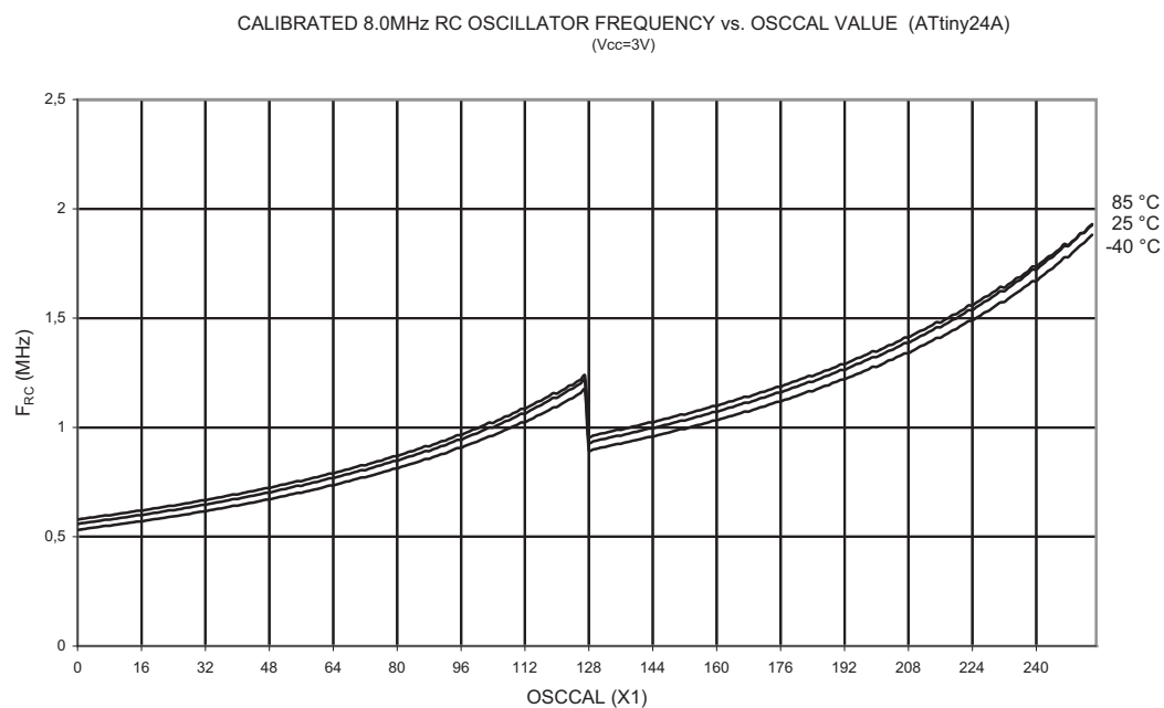
Figure 21-54. Calibrated 8 MHz RC Oscillator Frequency vs. OSCCAL Value
