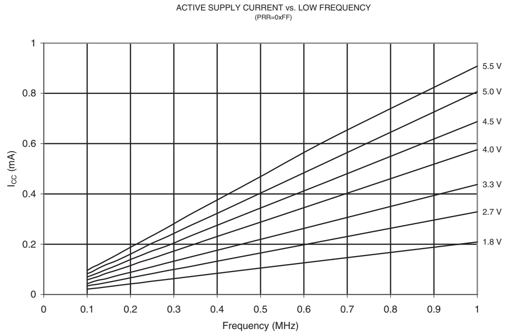
Figure 21-55. Active Supply Current vs. Low Frequency (0.1 - 1.0 MHz)
