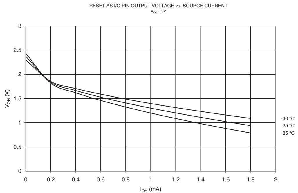
Figure 21-88. V_{OH} : Output Voltage vs. Source Current (Reset Pin as I/O, V_{CC} = 3V )
