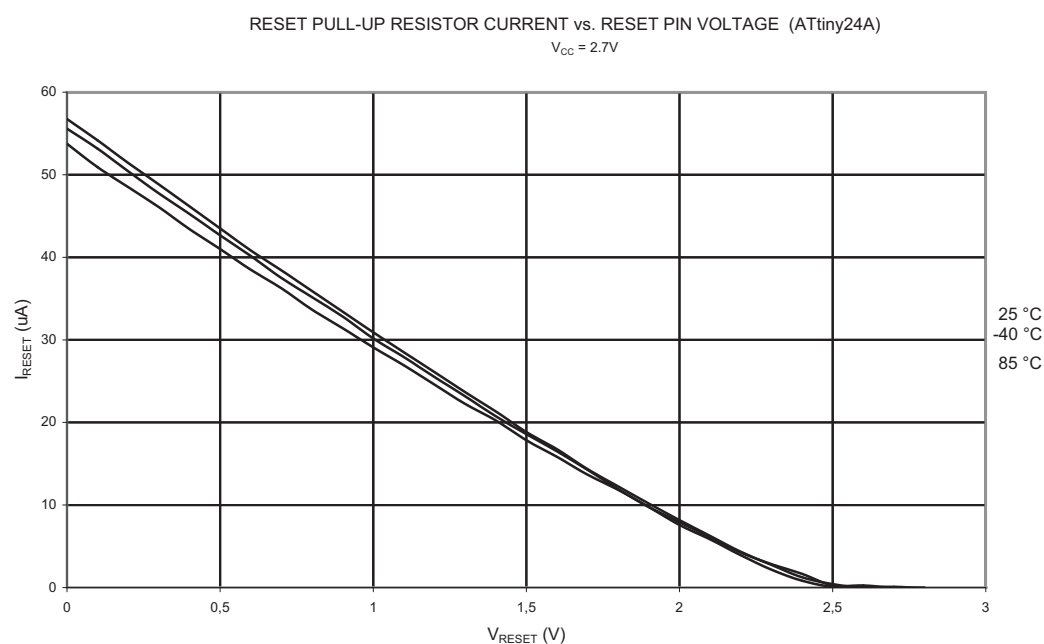
Figure 21-25. Reset Pull-up Resistor Current vs. Reset Pin Voltage ( V_{CC} = 2.7V )
