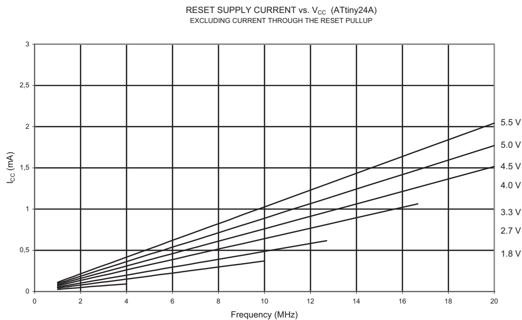
Figure 21-14. Reset Supply Current vs. V_{CC} (1 - 20 MHz, Excluding Current Through the Reset Pull-up)
