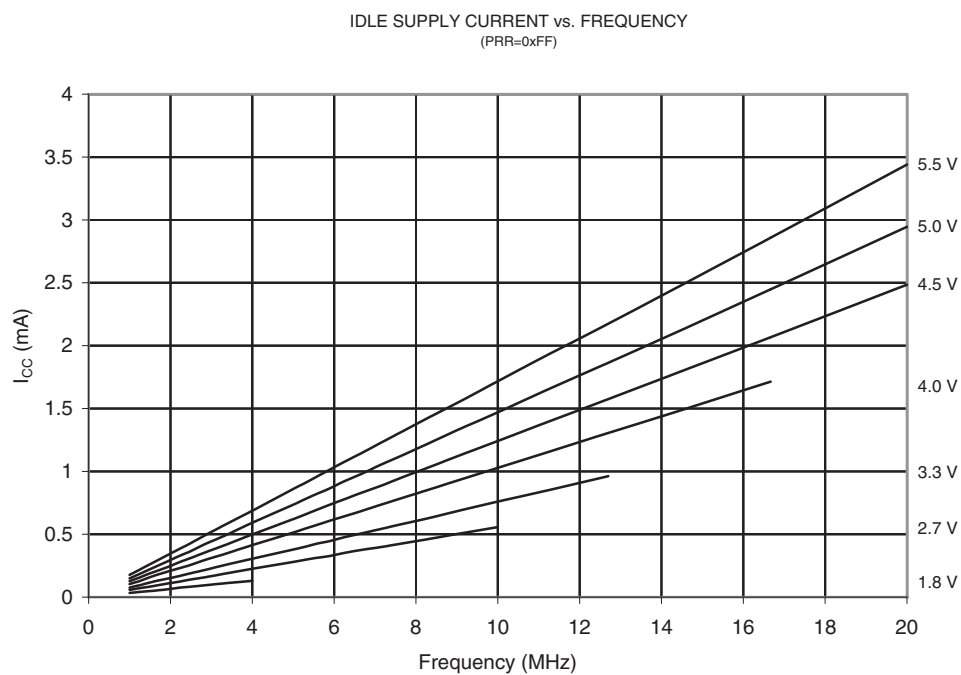
Figure 21-61. Idle Supply Current vs. Frequency (1 - 20 MHz)
