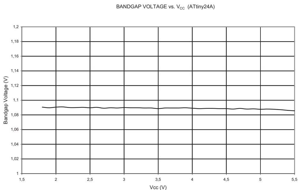
Figure 21-44. Bandgap Voltage vs. Supply Voltage
