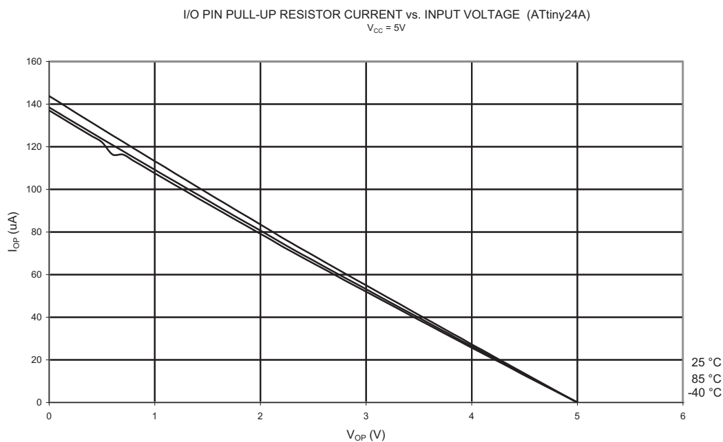
Figure 21-23. Pull-up Resistor Current vs. Input Voltage (I/O Pin, V_{CC} = 5V )
