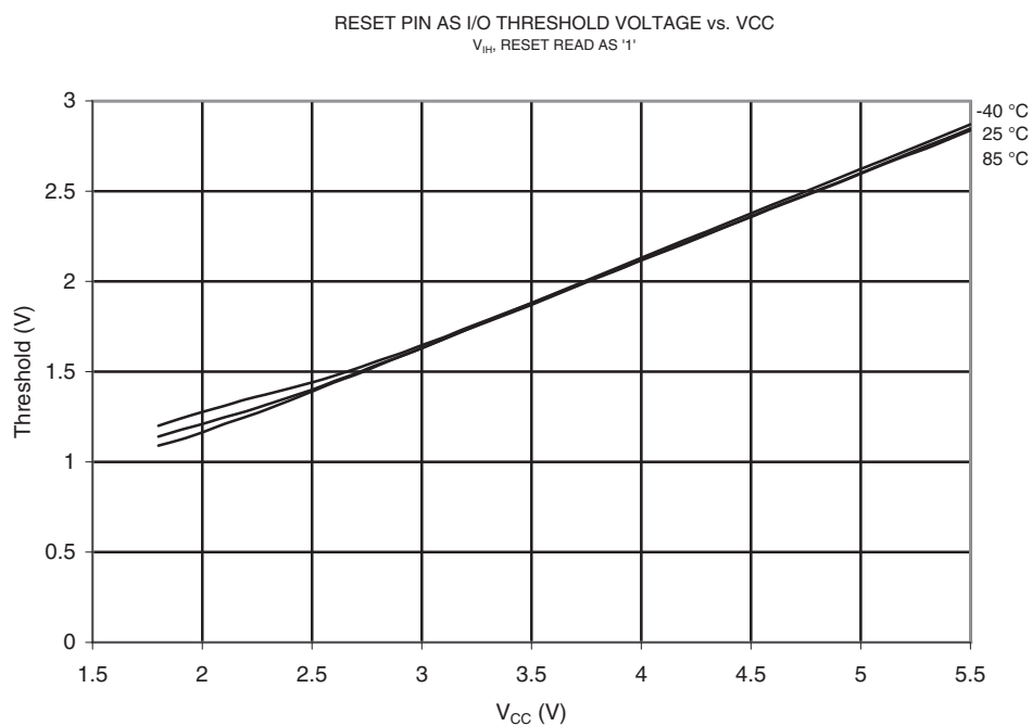
Figure 21-93. V_{IH} : Input Threshold Voltage vs. V_{CC} (Reset Pin as I/O, Read as '1')
