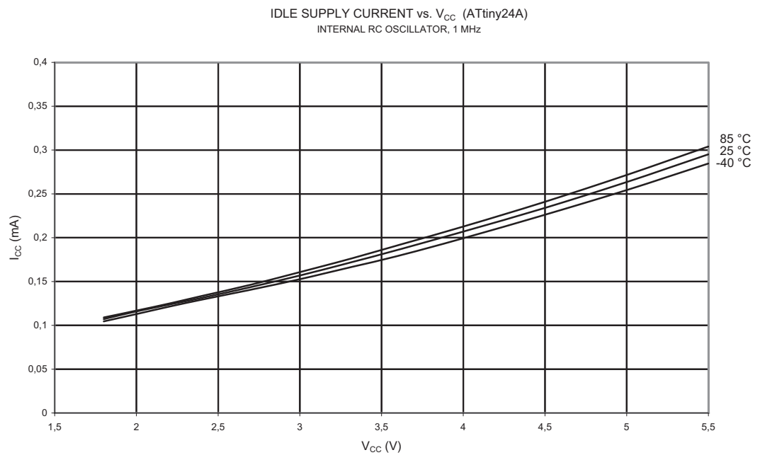
Figure 21-9. Idle Supply Current vs. V_{CC} (Internal RC Oscillator, 1 MHz)
