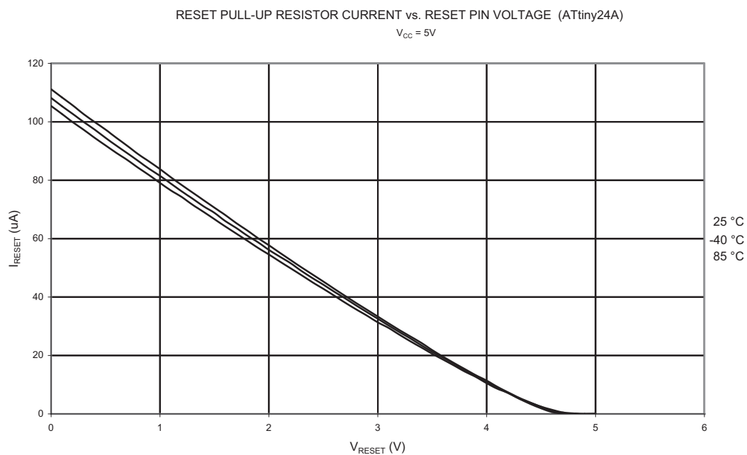
Figure 21-26. Reset Pull-up Resistor Current vs. Reset Pin Voltage ( V_{CC} = 5V )
