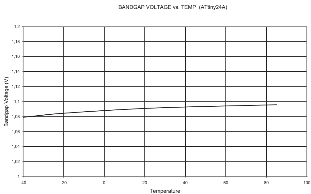
Figure 21-45. Bandgap Voltage vs. Temperature
