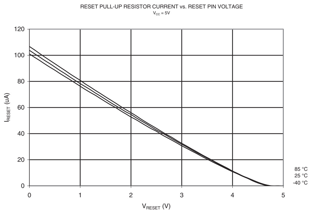
Figure 21-81. Reset Pull-up Resistor Current vs. Reset Pin Voltage ( V_{CC} = 5V )
