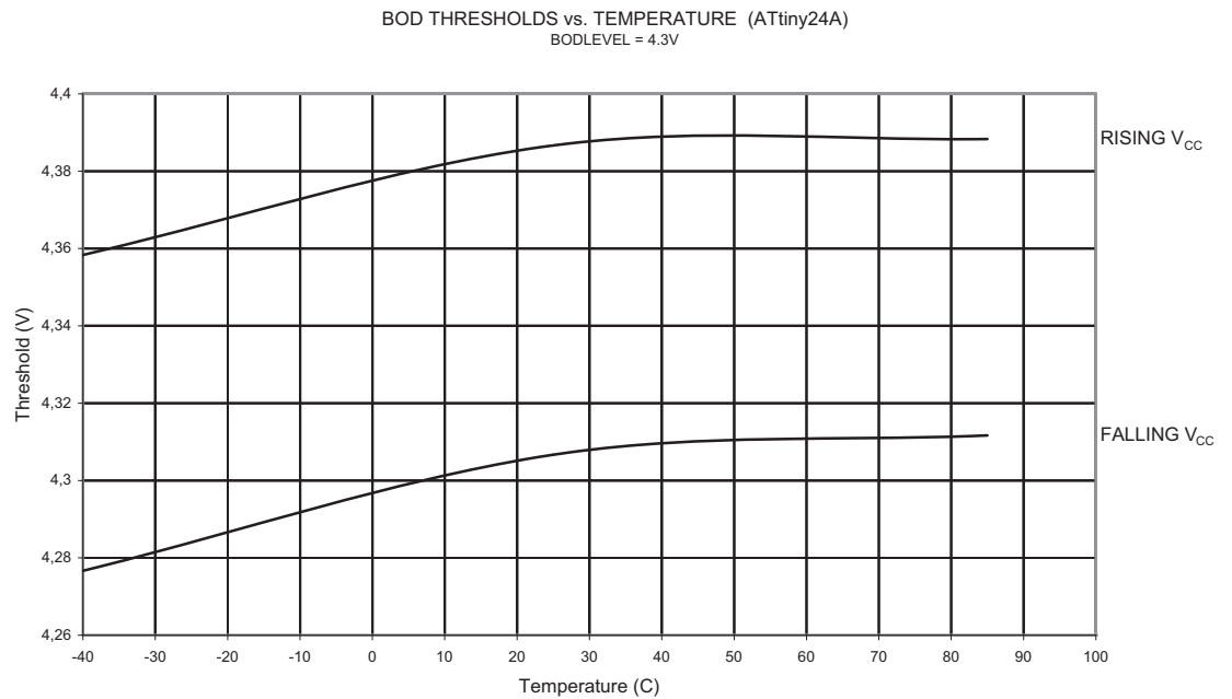
Figure 21-41. BOD Threshold vs. Temperature (BODLEVEL is 4.3V)
