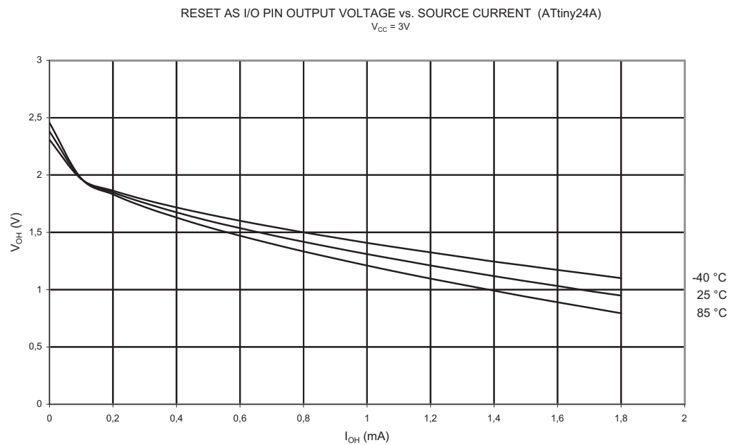
Figure 21-33. V_{OH} : Output Voltage vs. Source Current (Reset Pin as I/O, V_{CC} = 3V )
