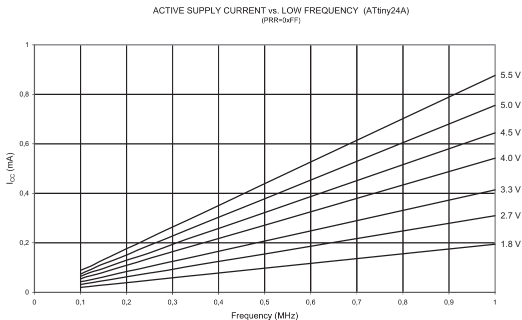
Figure 21-1. Active Supply Current vs. Low Frequency (0.1 - 1.0 MHz)
