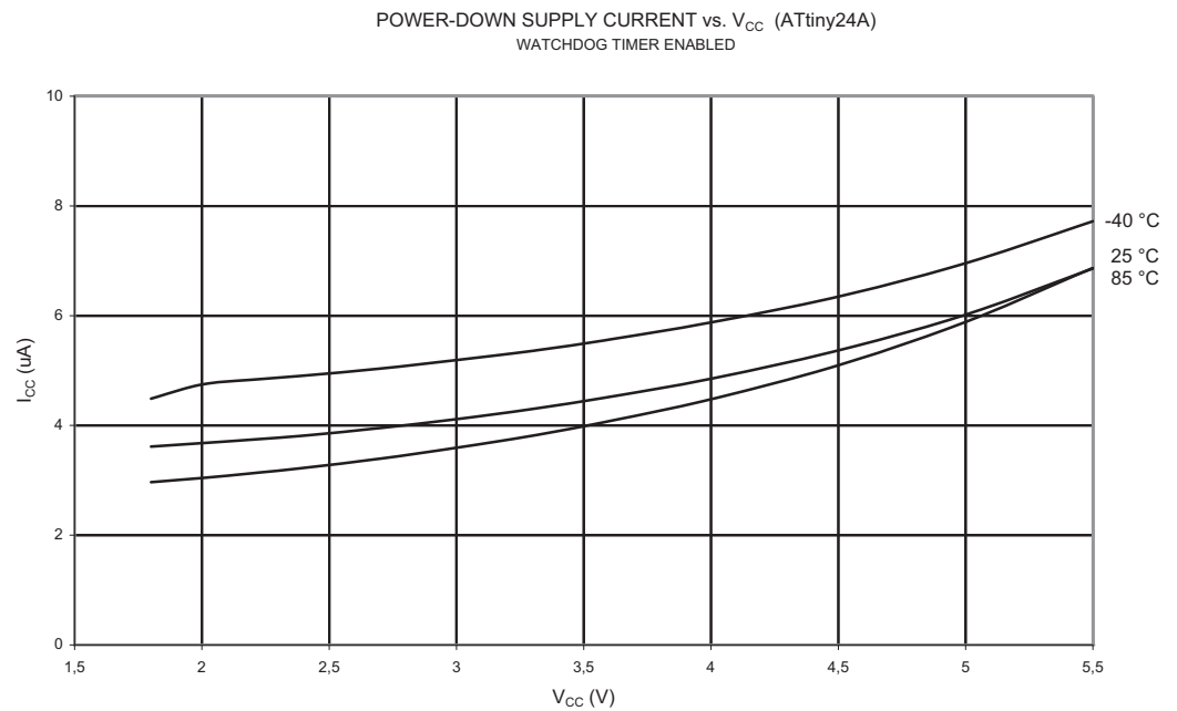
Figure 21-12. Power-down Supply Current vs. V_{CC} (Watchdog Timer Enabled)
