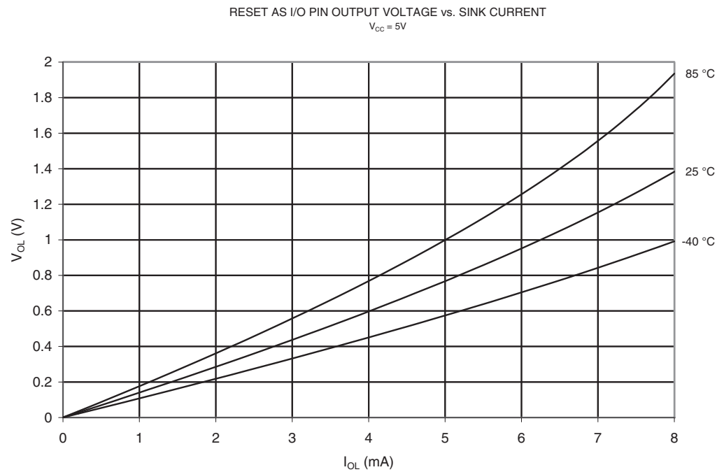
Figure 21-87. V_{OL} : Output Voltage vs. Sink Current (Reset Pin as I/O, V_{CC} = 5V )
