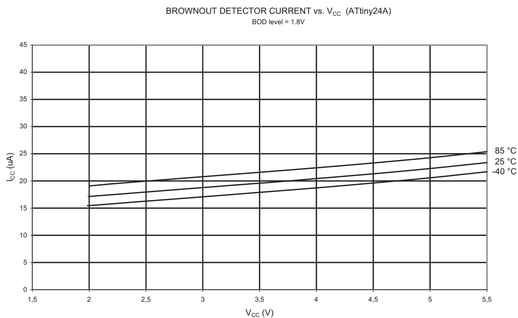
Figure 21-19. Brownout Detector Current vs. V_{CC}
