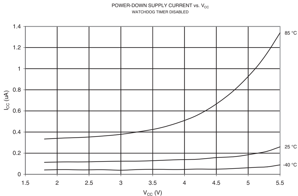
Figure 21-65. Power-down Supply Current vs. V_{CC} (Watchdog Timer Disabled)
