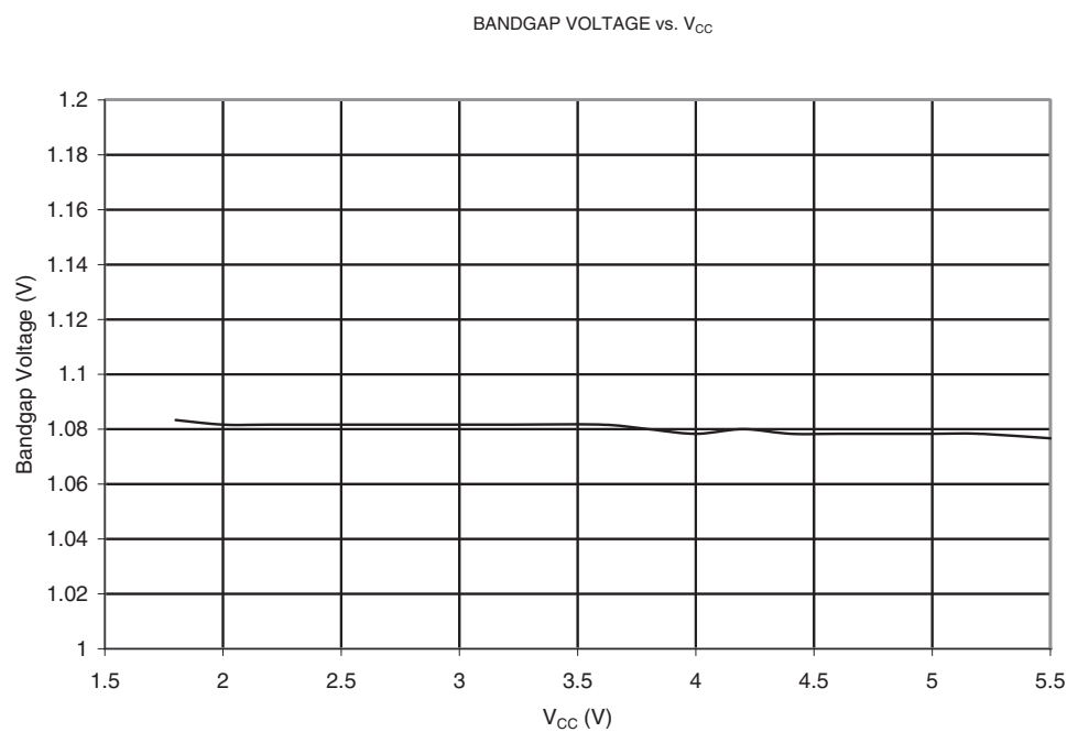
Figure 21-99. Internal Bandgap Voltage vs. Supply Voltage
