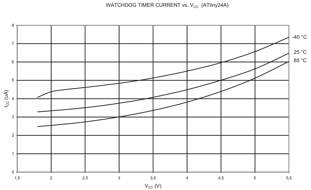
Figure 21-20. Watchdog Timer Current vs. V_{CC}
