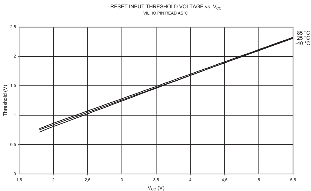
Figure 21-102. V_{IL} : Input Threshold Voltage vs. V_{CC} (Reset Pin, Read as '0')
