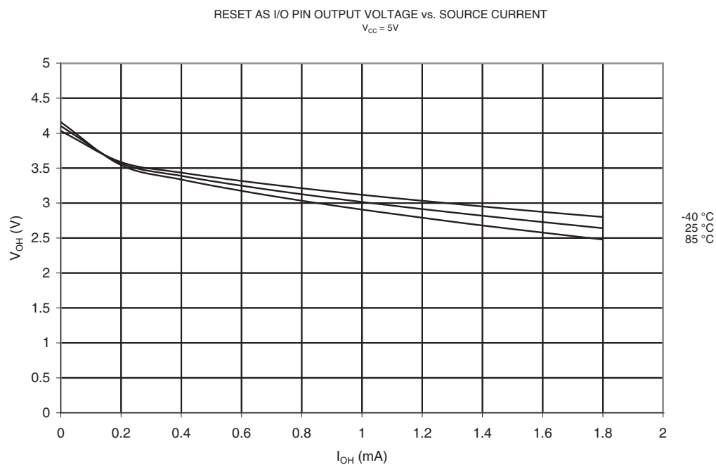
Figure 21-89. V_{OH} : Output Voltage vs. Source Current (Reset Pin as I/O, V_{CC} = 5V )
