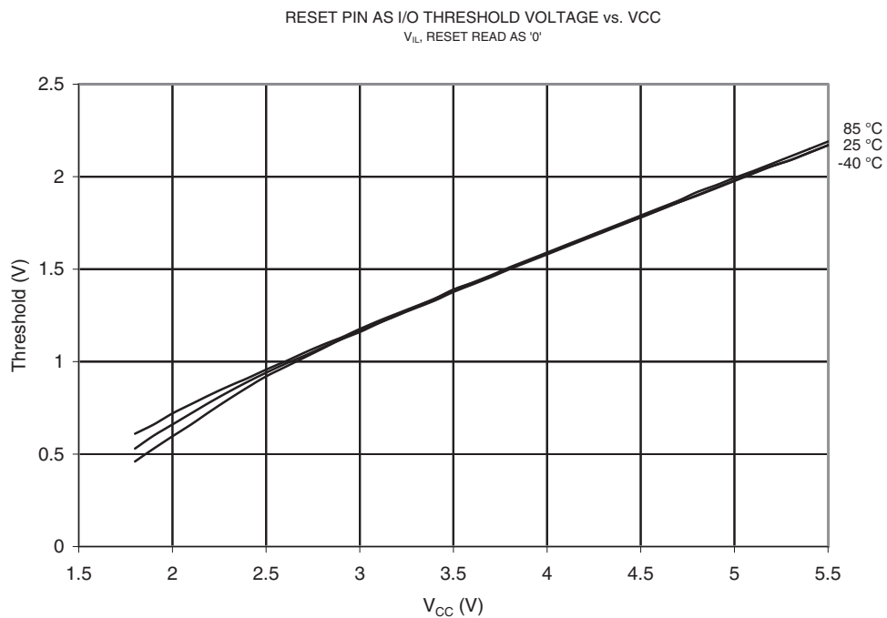
Figure 21-94. V_{IL} : Input Threshold Voltage vs. V_{CC} (Reset Pin as I/O, Read as '0')
