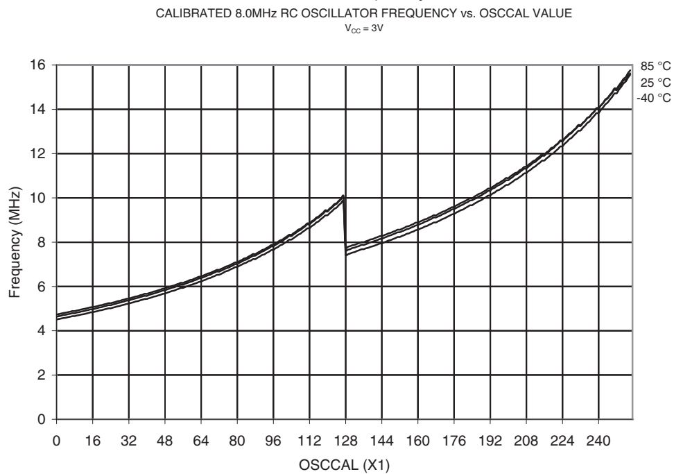
Figure 21-109. Calibrated 8 MHz RC Oscillator Frequency vs, OSCCAL Value
