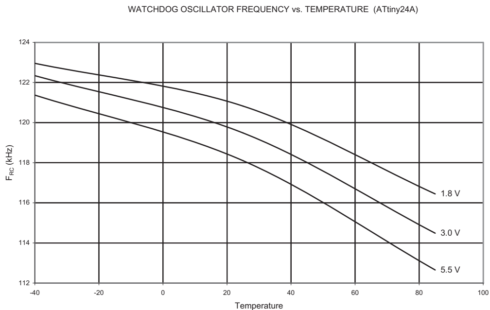
Figure 21-51. Watchdog Oscillator Frequency vs. Temperature
