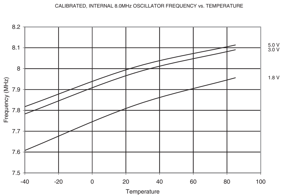
Figure 21-108. Calibrated 8 MHz RC oscillator Frequency vs. Temperature
