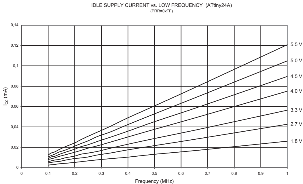
Figure 21-6. Idle Supply Current vs. Low Frequency (0.1 - 1.0 MHz)
