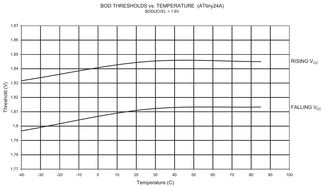
Figure 21-43. BOD Threshold vs. Temperature (BODLEVEL is 1.8V)
