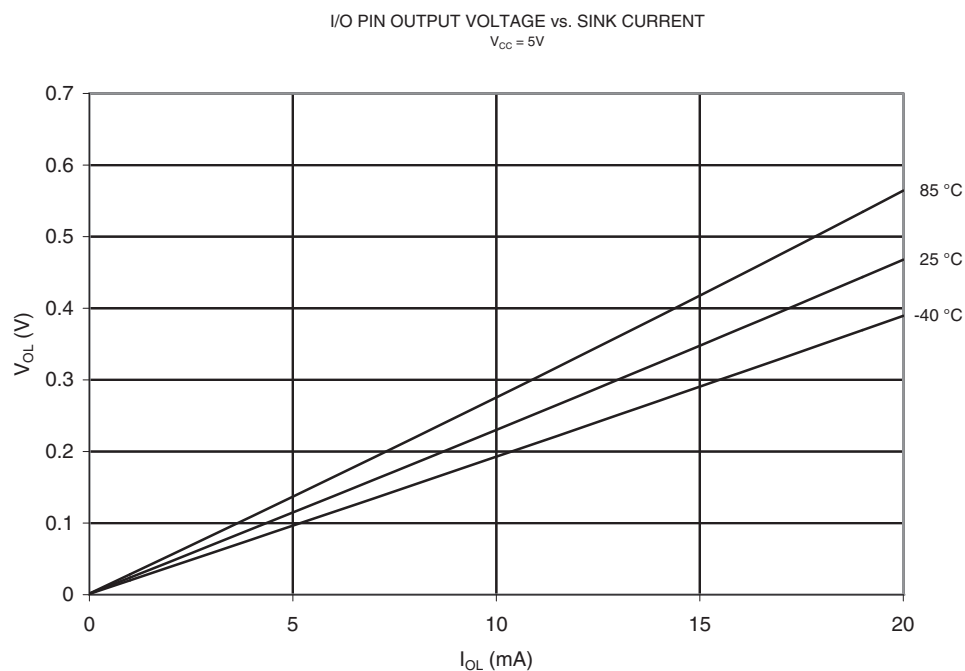
Figure 21-83. V_{OL} : Output Voltage vs. Sink Current (I/O Pin, V_{CC} = 5V )
