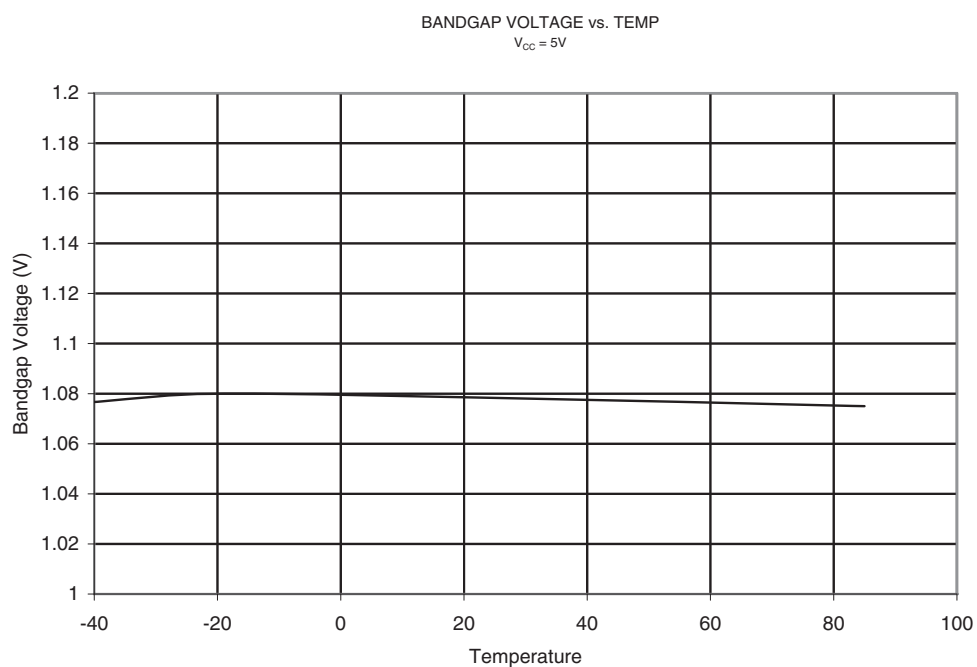
Figure 21-100. Internal Bandgap Voltage vs. Temperature
