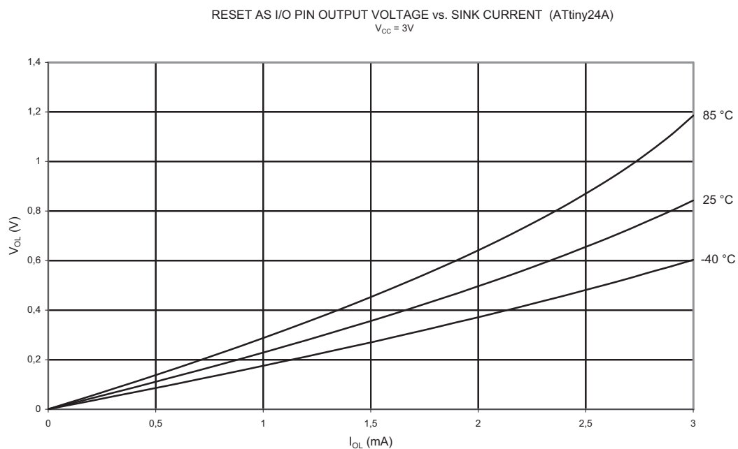
Figure 21-31. V_{OL} : Output Voltage vs. Sink Current (Reset Pin as I/O, V_{CC} = 3V )
