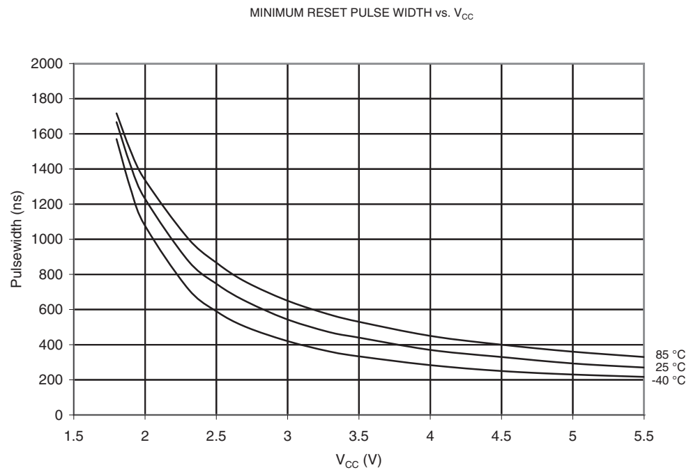
Figure 21-104. Minimum Reset Pulse Width vs. V_{CC}
