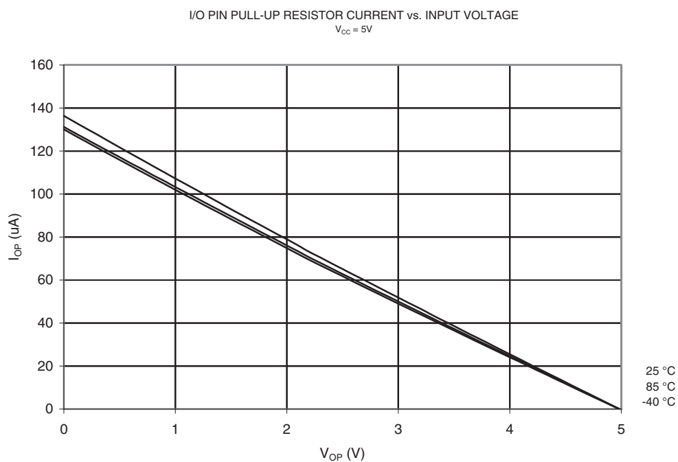
Figure 21-78. Pull-up Resistor Current vs. Input Voltage (I/O Pin, V_{CC} = 5V )
