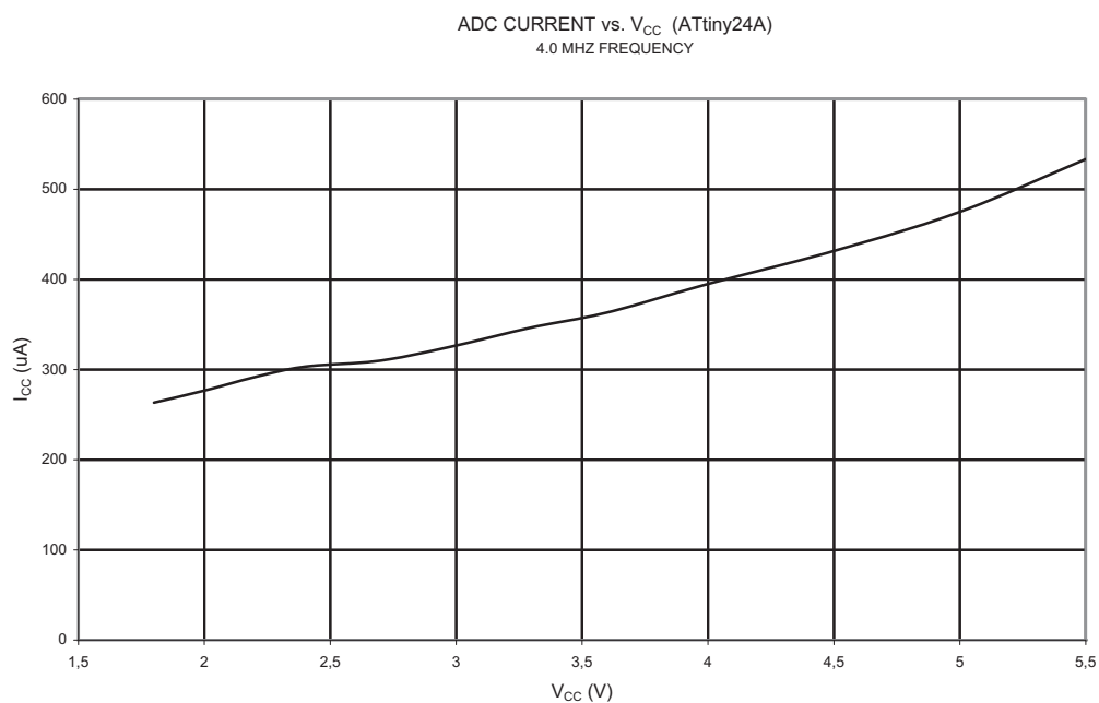
Figure 21-15. ADC Current vs. V_{CC}
