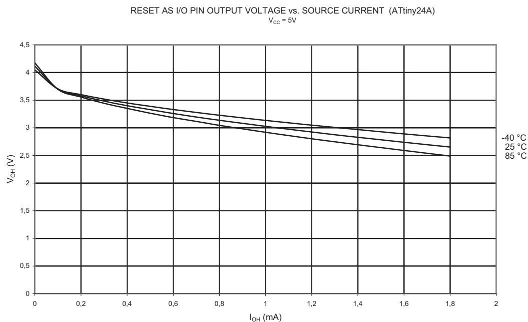
Figure 21-34. V_{OH} : Output Voltage vs. Source Current (Reset Pin as I/O, V_{CC} = 5V )
