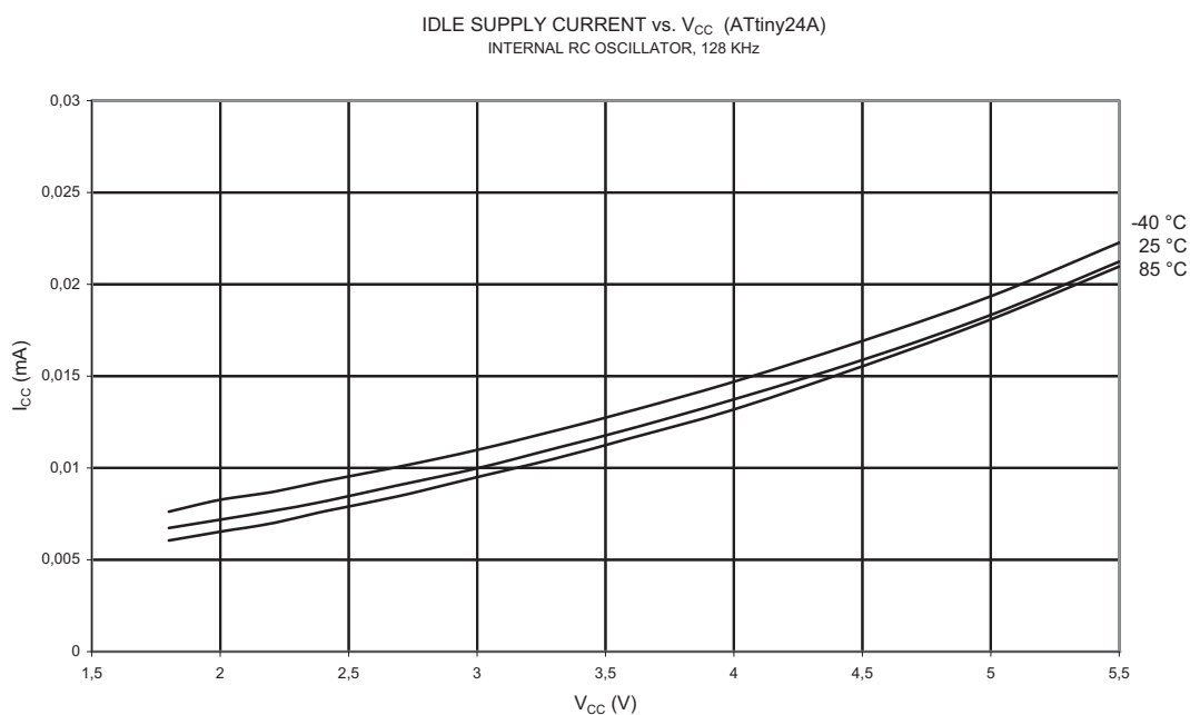
Figure 21-10. Idle Supply Current vs. V_{CC} (Internal RC Oscillator, 128 kHz)
