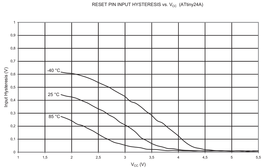
Figure 21-48. V_{IH} - V_{IL} : Input Hysteresis vs. V_{CC} (Reset Pin)
