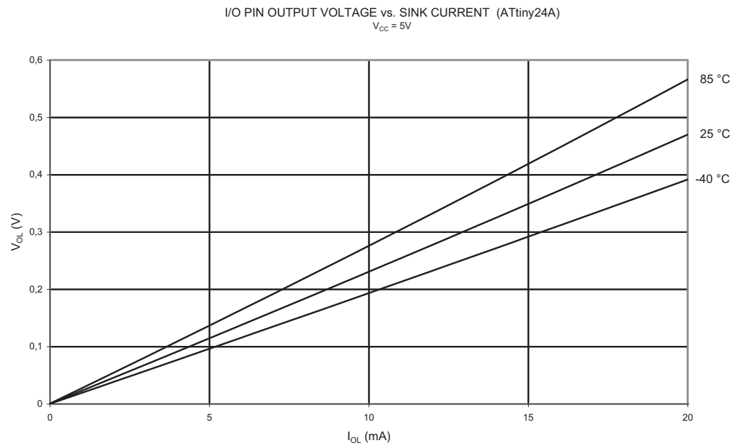
Figure 21-28. V_{OL} : Output Voltage vs. Sink Current (I/O Pin, V_{CC} = 5V )
