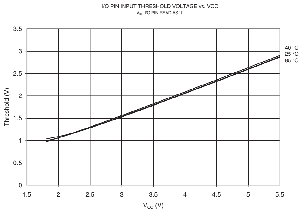
Figure 21-90. V_{IH} : Input Threshold Voltage vs. V_{CC} (IO Pin, Read as '1')
