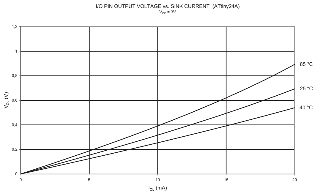
Figure 21-27. V_{OL} : Output Voltage vs. Sink Current (I/O Pin, V_{CC} = 3V )
