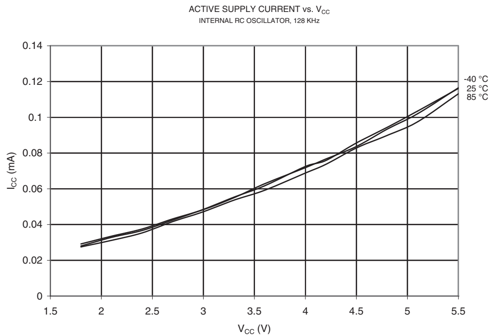
Figure 21-59. Active Supply Current vs. V_{CC} (Internal RC Oscillator, 128 kHz)
