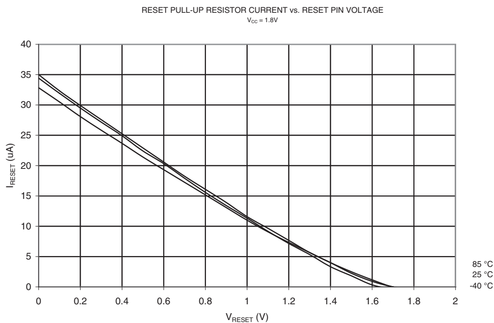
Figure 21-79. Reset Pull-up Resistor Current vs. Reset Pin Voltage ( V_{CC} = 1.8V )
