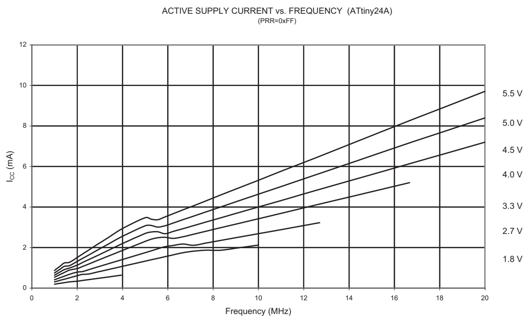
Figure 21-2. Active Supply Current vs. frequency (1 - 20 MHz)
