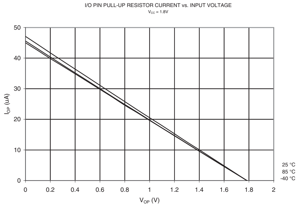
Figure 21-76. Pull-up Resistor Current vs. Input Voltage (I/O Pin, V_{CC} = 1.8V )
