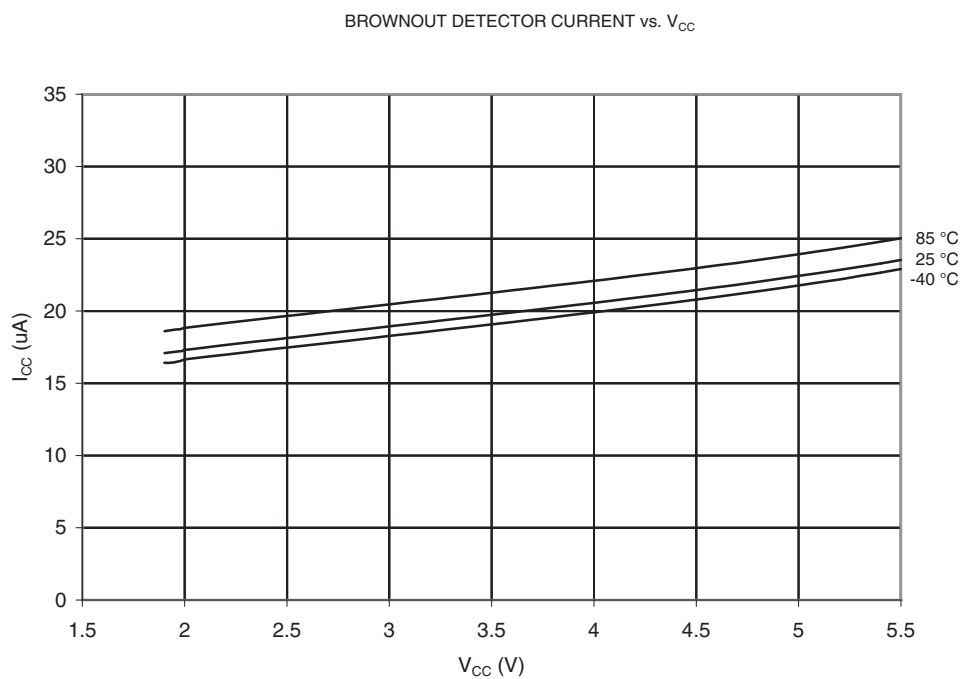
Figure 21-73. Brownout Detector Current vs. V_{CC}
