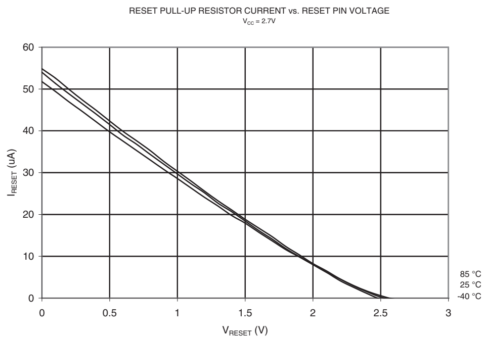
Figure 21-80. Reset Pull-up Resistor Current vs. Reset Pin Voltage ( V_{CC} = 2.7V )
