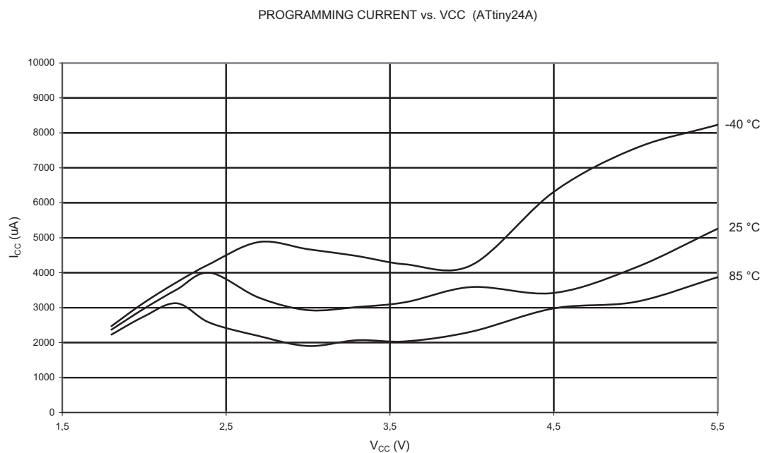
Figure 21-18. Programming Current vs. V_{CC}
