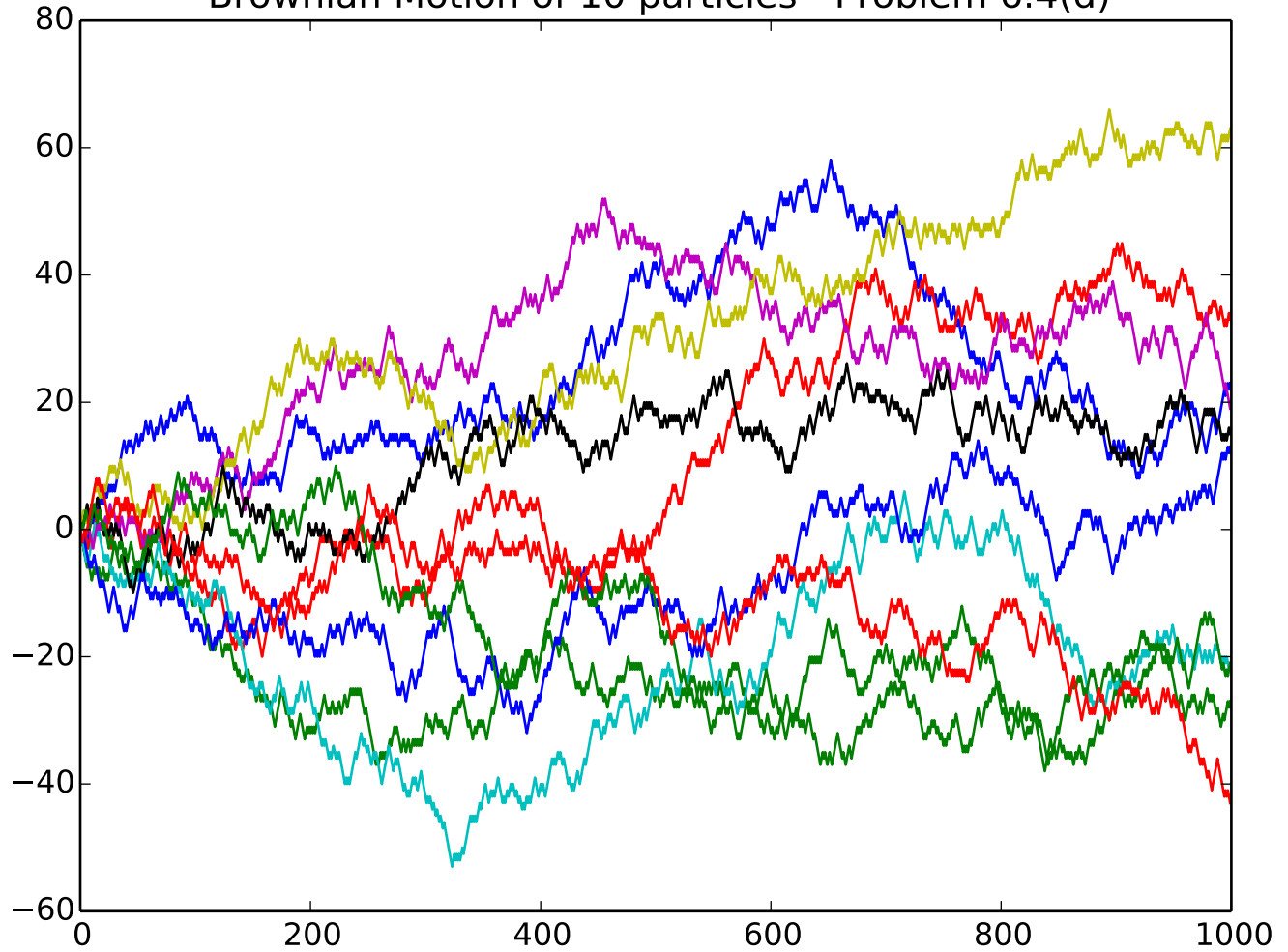
Brownian Motion of 10 particles - Problem 6.4(d)
