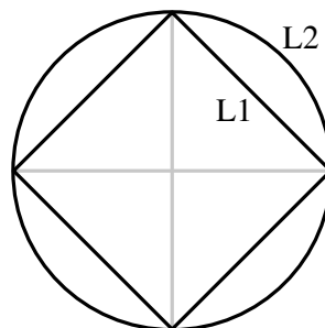
Figure 13.3. Constant L1 and L2 norms.
