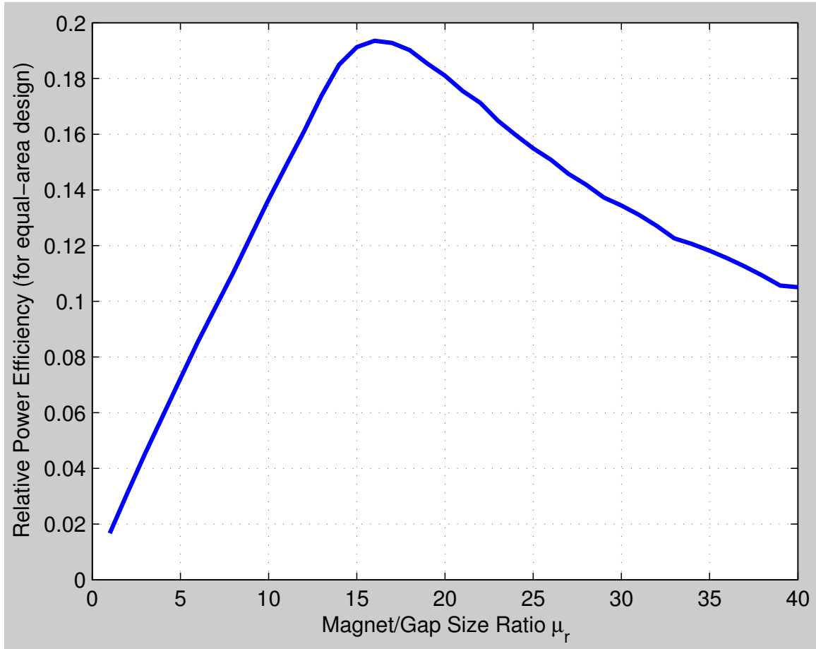
Figure 5-23: Relative power efficiency vs size ratio. The relative power efficiency is the ratio of the mechanical work done by the gap closing to the hysteresis loss of the Alnico magnet. The magnet/gap size ratio \mu_r is defined in the text. This plot is valid only for a design with equal magnet and pole area; in that case, the magnet/gap size ratio is the ratio of the total magnet length on the flux path to the length of the air gap.
