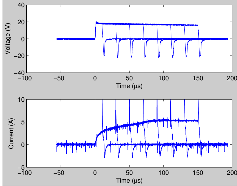
Figure 5-13: Electropermanent actuator pulse voltage and current vs. time. In the figures above, we have overlaid the plots for eight linearly-spaced pulse lengths from 10 \mu s - 150 \mu s . Demonstrating the causality and repeatability of the system, the pulses follow identical trajectories until the voltage is turned off, when a negative-voltage spike corresponding to the partial collapse of the magnetic field is observed.
