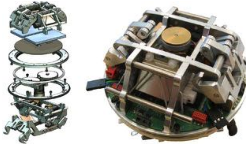
Figure 2-8: ATRON module mechanics. (Østergaard [71])
