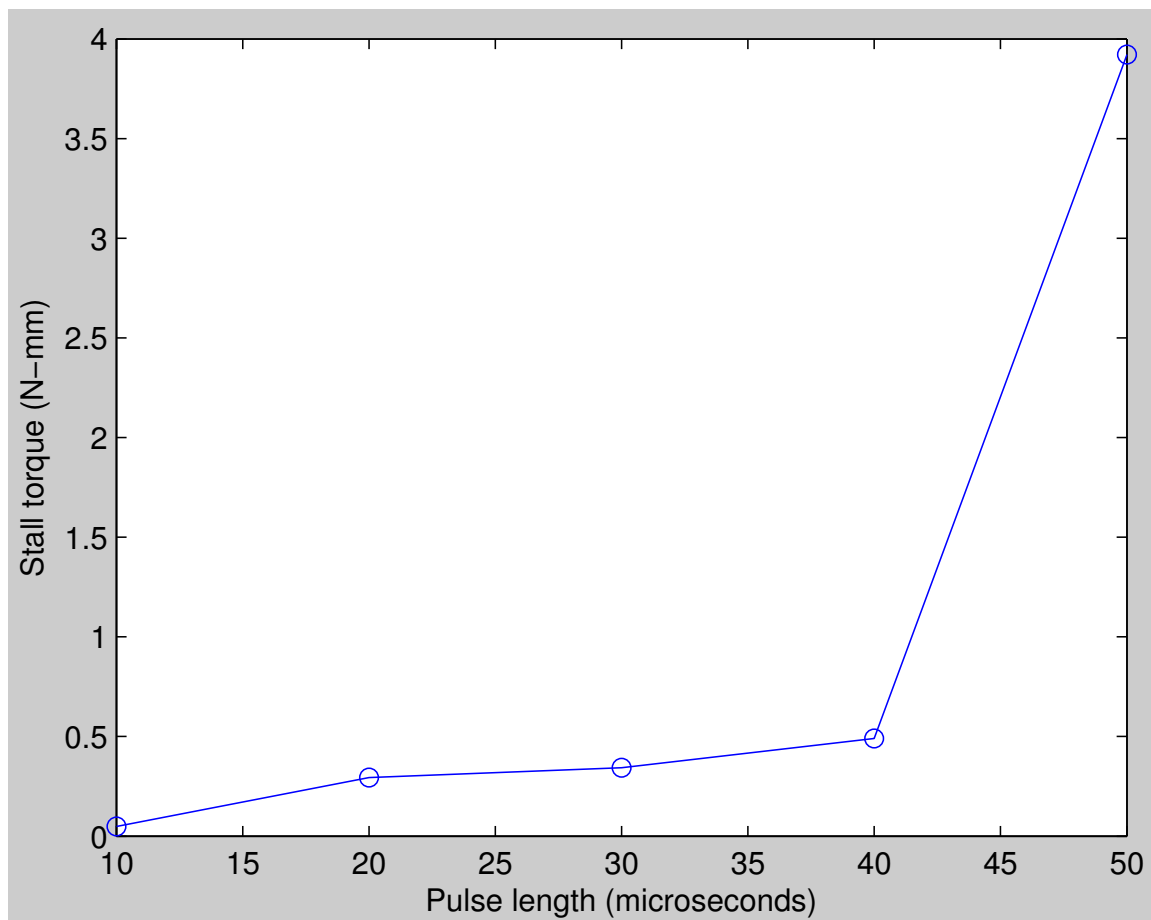
Figure 5-26: Electropermanent stepper torque vs. pulse length, measured by hanging weights on a string from the rotor until the backdriving occurred. This plot shows that the stall torque of the motor is considerably higher than its dynamic torque and that the torque can be controlled by the driving pulse length.
