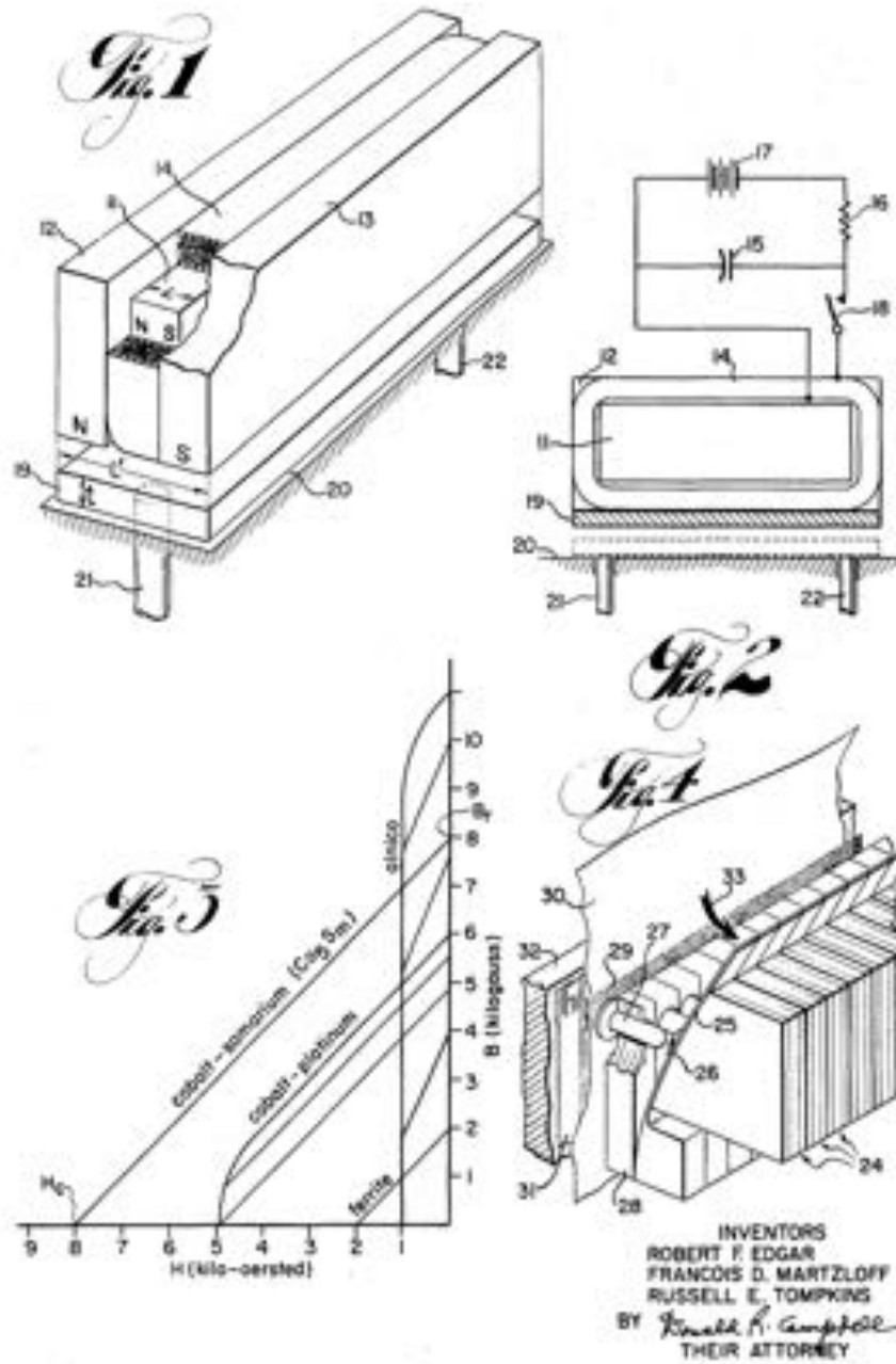
Figure 2-25: Monostable electropermanent magnet based on the flux-cancellation principle. (Edgar [21])
