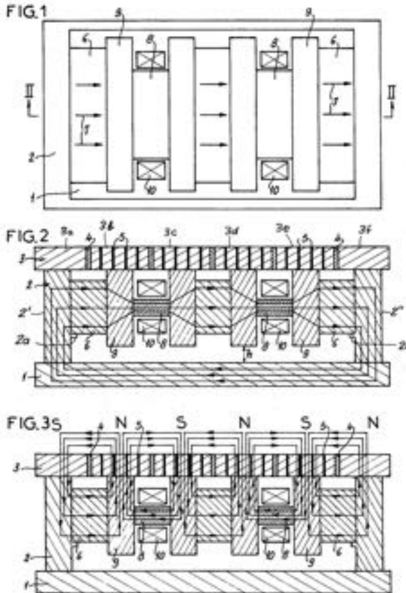
Figure 2-27: Series electropermanent magnet for magnetic workholding. With all the magnets magnetized in the same direction, flux travels through the bottom plate. (Fig. 2) With every second magnet oppositely magnetized, flux circulates locally, holding down the workpiece. (Fig. 3) (Brailon [8])
