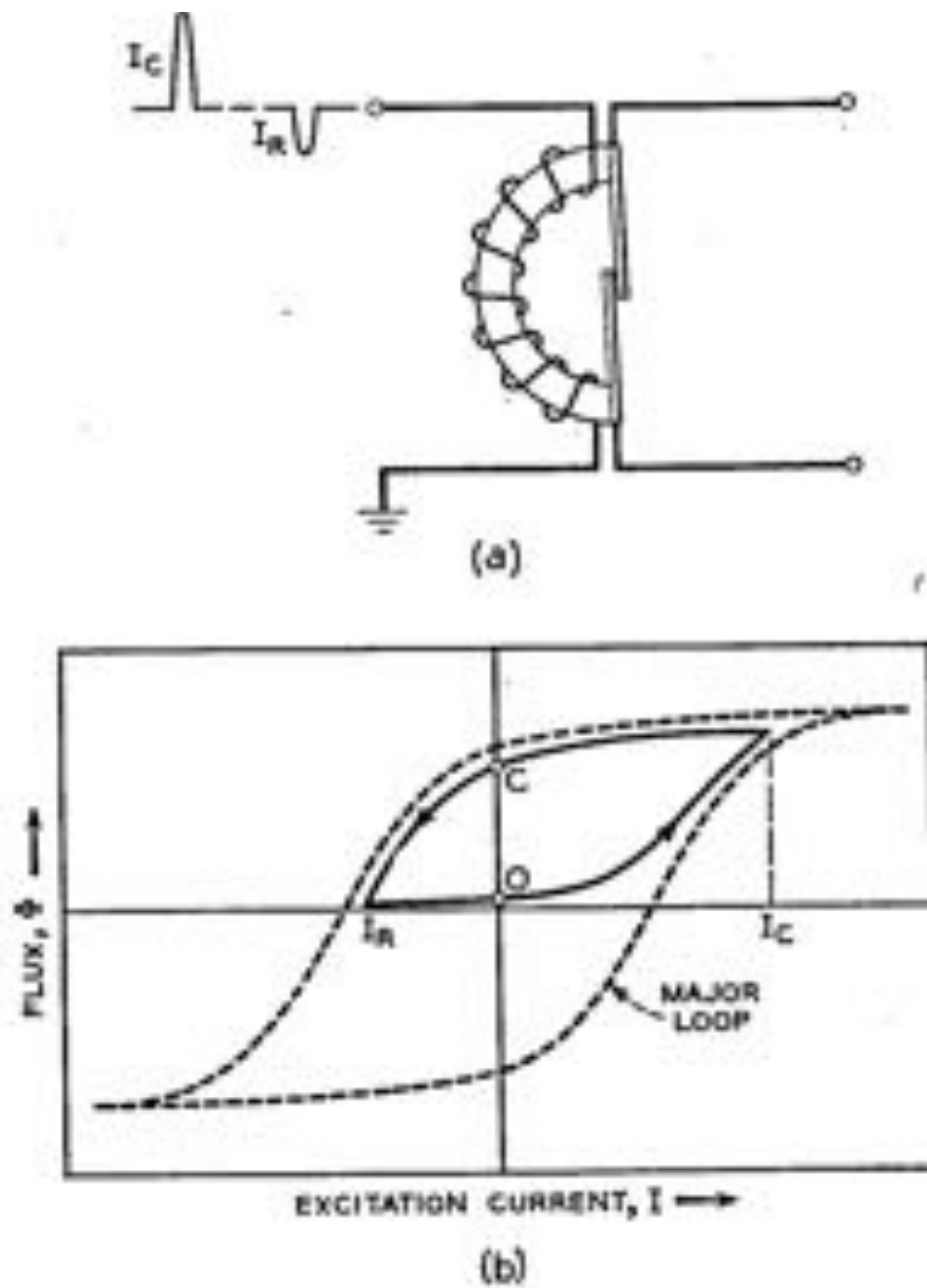
Figure 2-22: (a) The single-branch ferreed (b) its magnetization characteristic. (Feiner [24])
