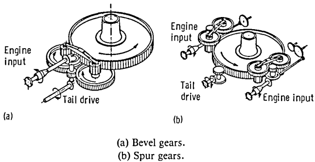
Figure 58.—Simple differentials.
