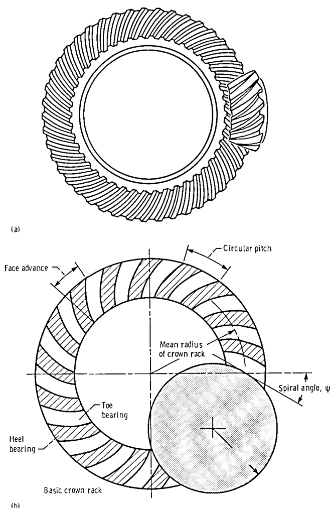
(a) Gear pair. (b) Cutting spiral gear teeth on basic crown rack.
