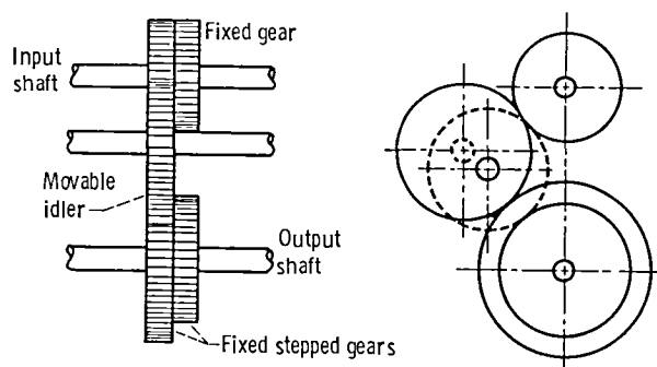
Figure 51.—Idler gear.
