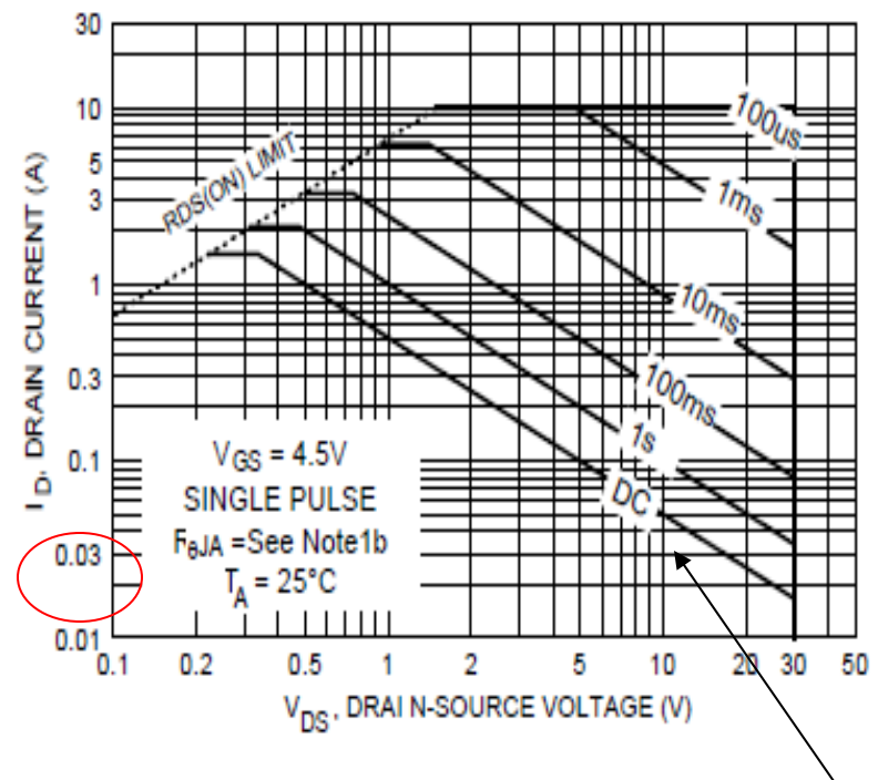
Figure 14. Maximum Safe Operating Area. 12V
