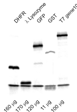
Figure 2. SDS-PAGE gel patterns of the products of the PURE system. After incubation of the translation reaction for 1 h in mixtures containing [ 35 S]methionine and 2.4 \mu\text{M} ribosome, samples were separated by SDS-PAGE and subjected to autoradiography. Below autoradiograph, yields calculated from the radioactivities of the labeled products and the productivity in 1 ml reaction. The bottom row of bands indicates the dye front.
